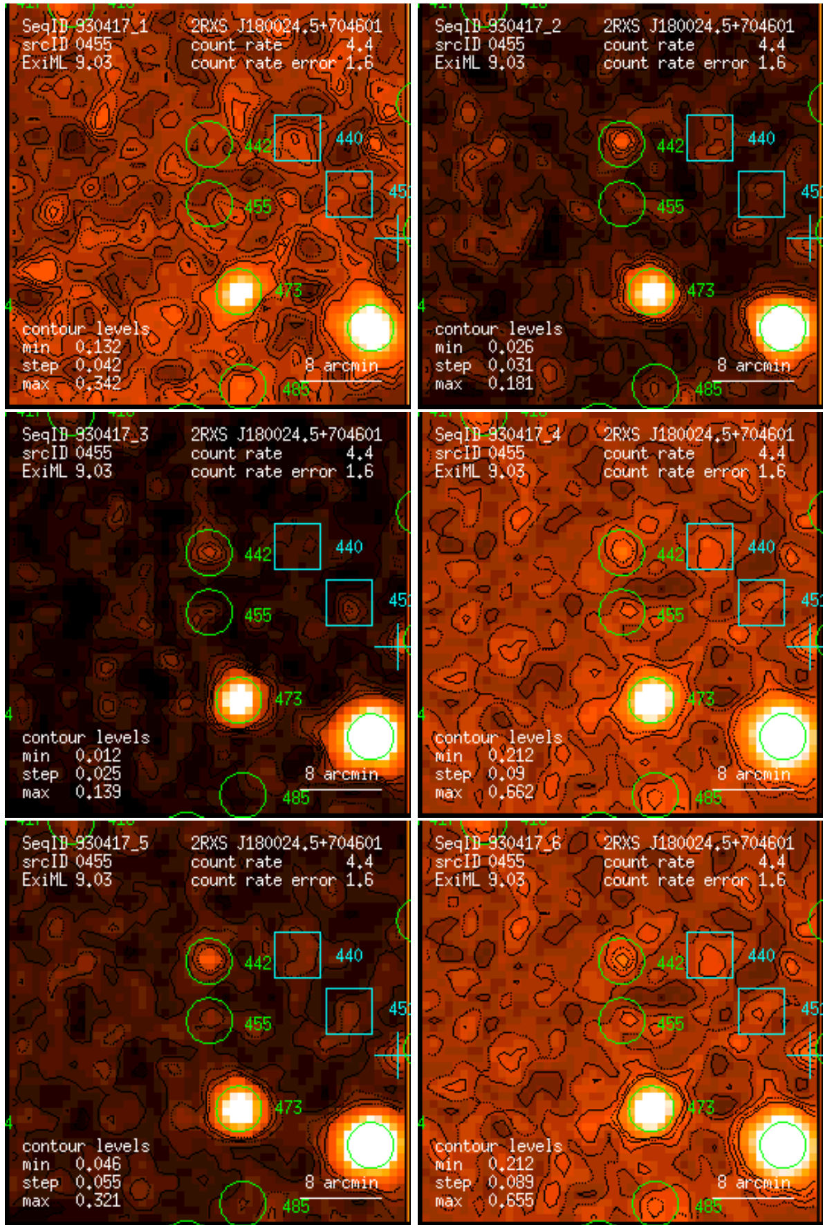
Figure 455: RASS 930417: detection 0455: band rate images, Gaussian filter: (1) PSPC channels 11 – 41, (2) 52 – 90, (3) 91 – 201, (4) 11 – 235, (5) 52 – 201, (6) 11 – 201. Broad band rates in counts/ks. Band rate contour levels in counts/ks/arcmin 2 .
