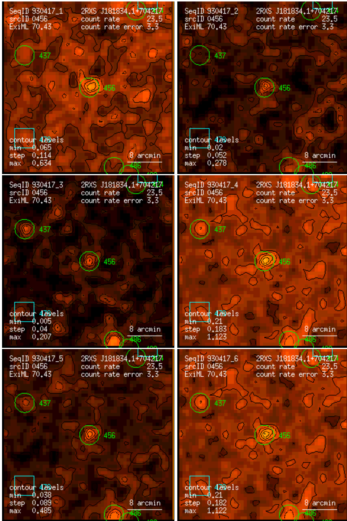
Figure 456: RASS 930417: detection 0456: band rate images, Gaussian filter: (1) PSPC channels 11 – 41, (2) 52 – 90, (3) 91 – 201, (4) 11 – 235, (5) 52 – 201, (6) 11 – 201. Broad band rates in counts/ks. Band rate contour levels in counts/ks/arcmin 2 .
