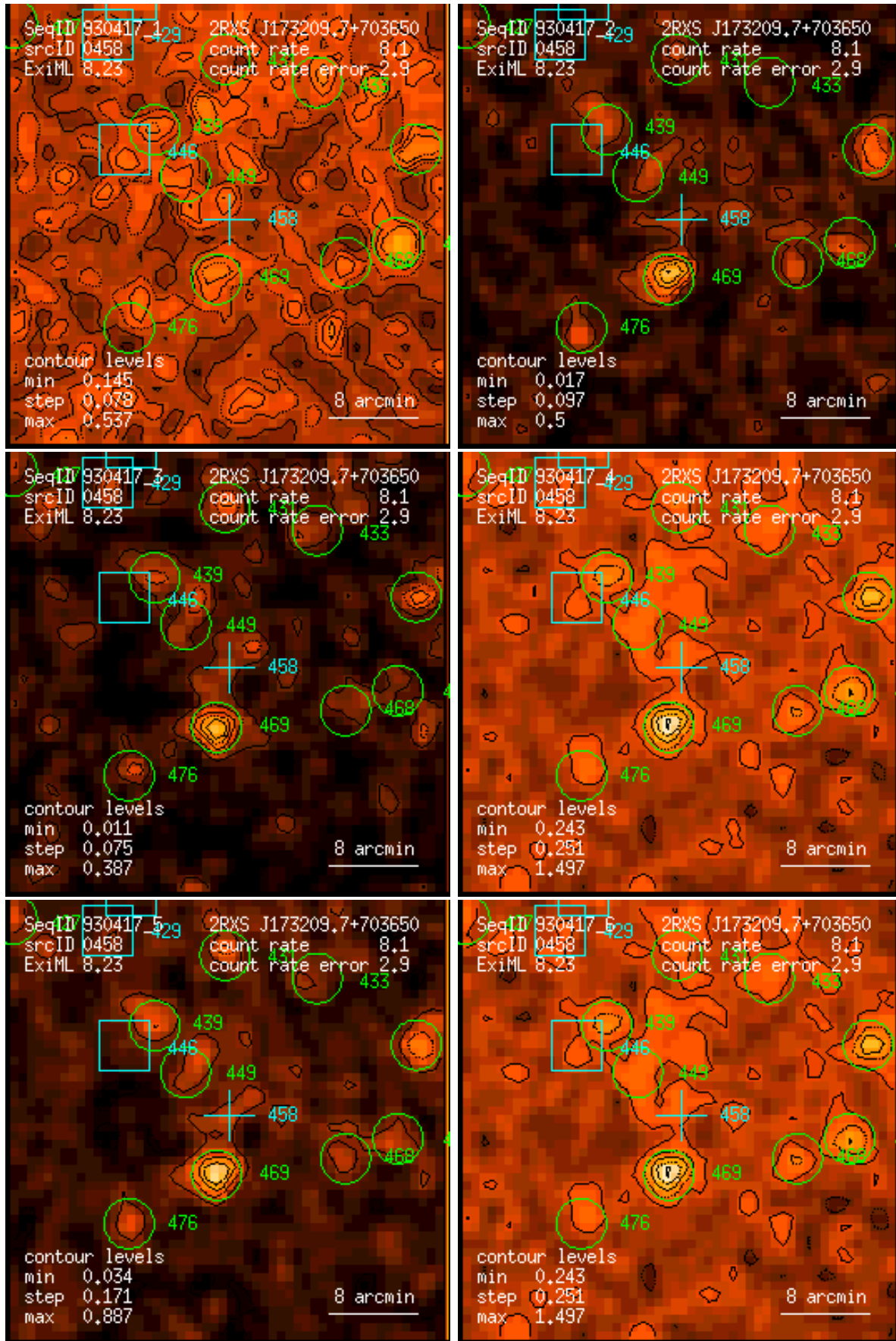
Figure 458: RASS 930417: detection 0458: band rate images, Gaussian filter: (1) PSPC channels 11 – 41, (2) 52 – 90, (3) 91 – 201, (4) 11 – 235, (5) 52 – 201, (6) 11 – 201. Broad band rates in counts/ks. Band rate contour levels in counts/ks/arcmin 2 .
