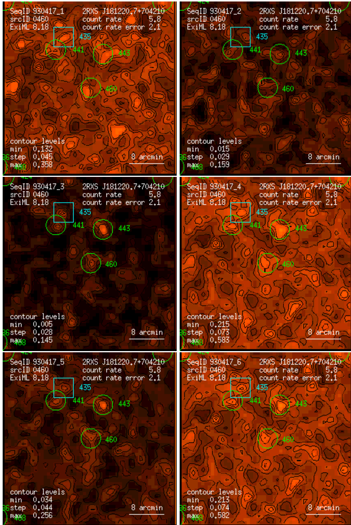
Figure 460: RASS 930417: detection 0460: band rate images, Gaussian filter: (1) PSPC channels 11 – 41, (2) 52 – 90, (3) 91 – 201, (4) 11 – 235, (5) 52 – 201, (6) 11 – 201. Broad band rates in counts/ks. Band rate contour levels in counts/ks/arcmin 2 .
