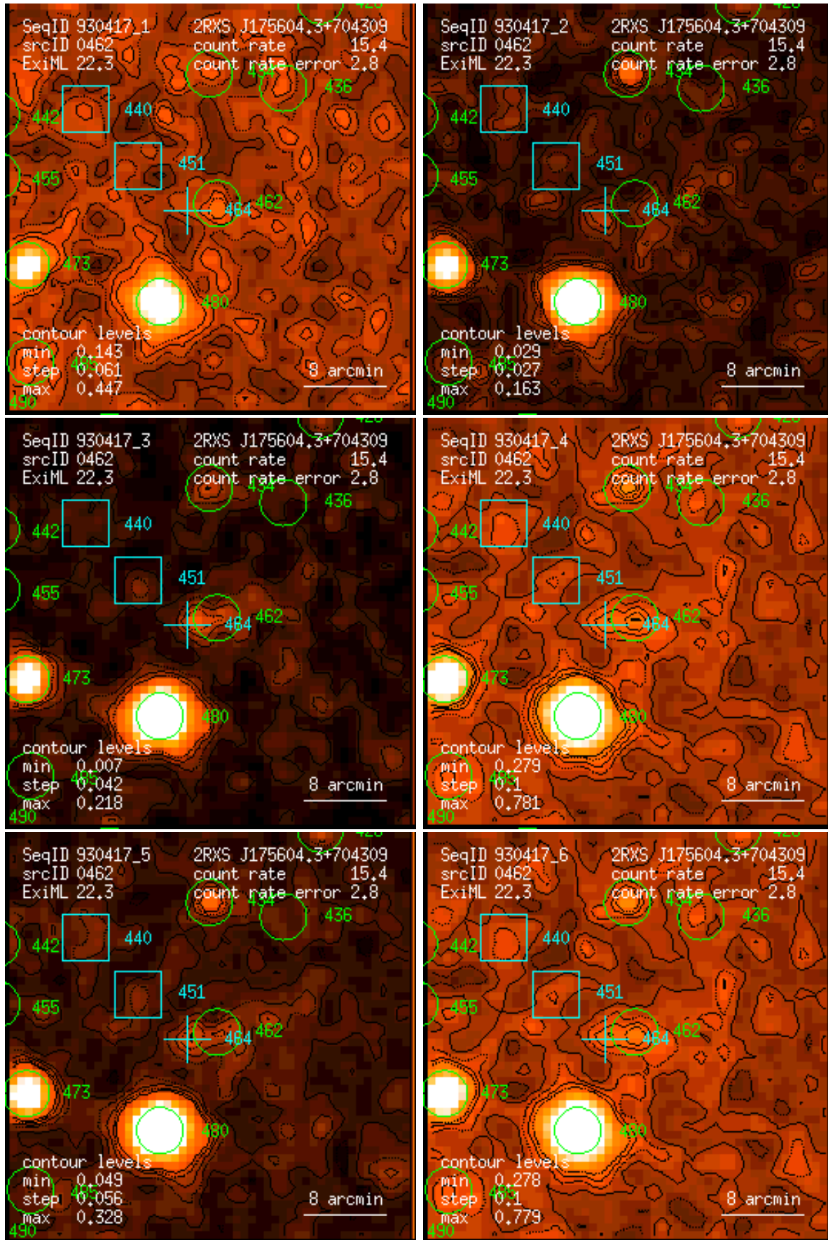
Figure 462: RASS 930417: detection 0462: band rate images, Gaussian filter: (1) PSPC channels 11 – 41, (2) 52 – 90, (3) 91 – 201, (4) 11 – 235, (5) 52 – 201, (6) 11 – 201. Broad band rates in counts/ks. Band rate contour levels in counts/ks/arcmin 2 .
