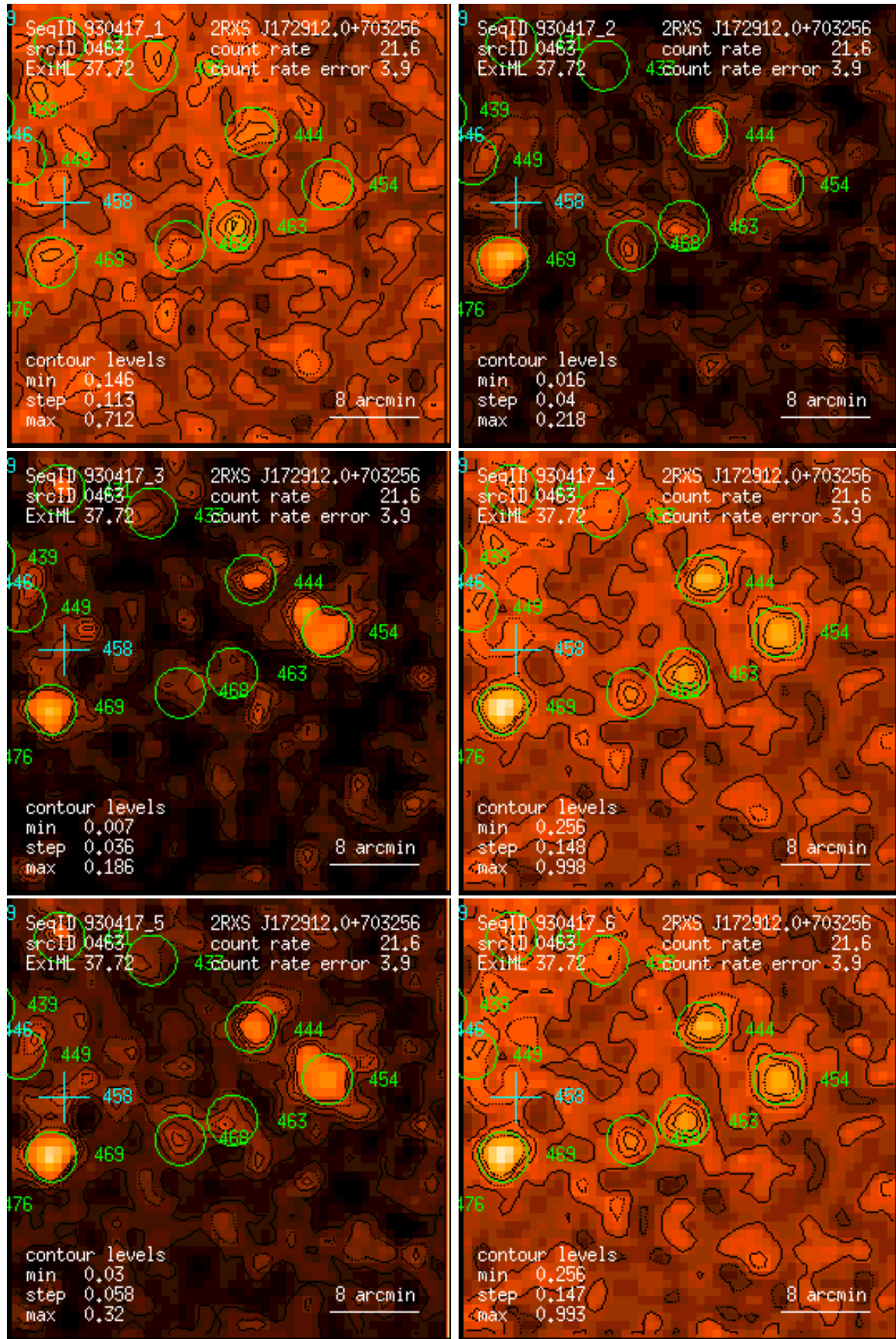
Figure 463: RASS 930417: detection 0463: band rate images, Gaussian filter: (1) PSPC channels 11 – 41, (2) 52 – 90, (3) 91 – 201, (4) 11 – 235, (5) 52 – 201, (6) 11 – 201. Broad band rates in counts/ks. Band rate contour levels in counts/ks/arcmin 2 .
