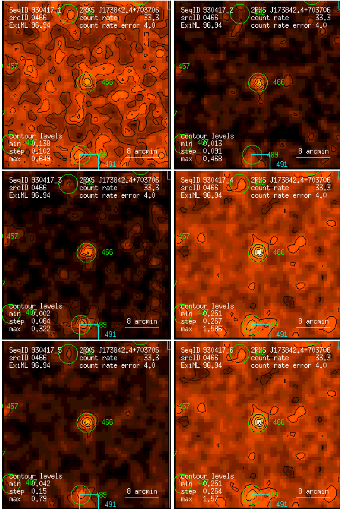
Figure 466: RASS 930417: detection 0466: band rate images, Gaussian filter: (1) PSPC channels 11 – 41, (2) 52 – 90, (3) 91 – 201, (4) 11 – 235, (5) 52 – 201, (6) 11 – 201. Broad band rates in counts/ks. Band rate contour levels in counts/ks/arcmin 2 .
