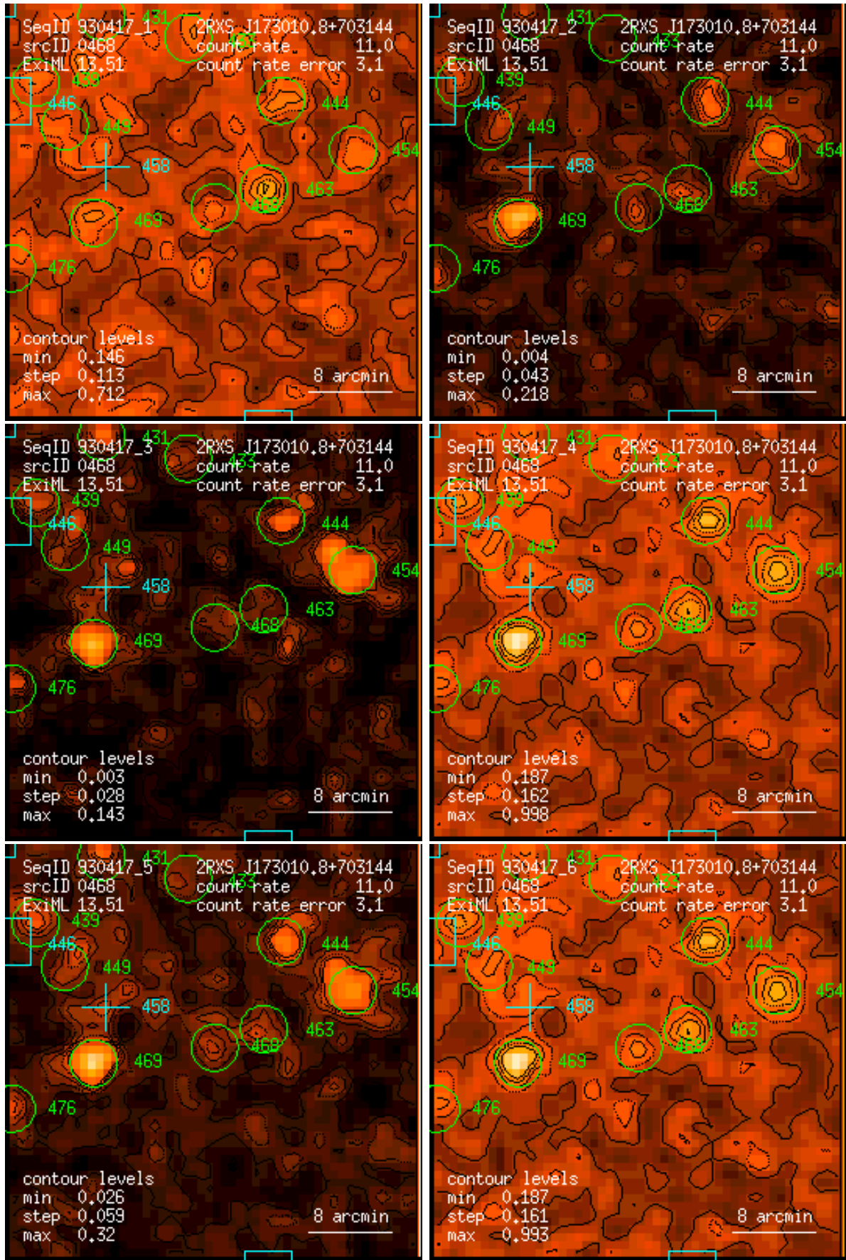
Figure 468: RASS 930417: detection 0468: band rate images, Gaussian filter: (1) PSPC channels 11 – 41, (2) 52 – 90, (3) 91 – 201, (4) 11 – 235, (5) 52 – 201, (6) 11 – 201. Broad band rates in counts/ks. Band rate contour levels in counts/ks/arcmin 2 .
