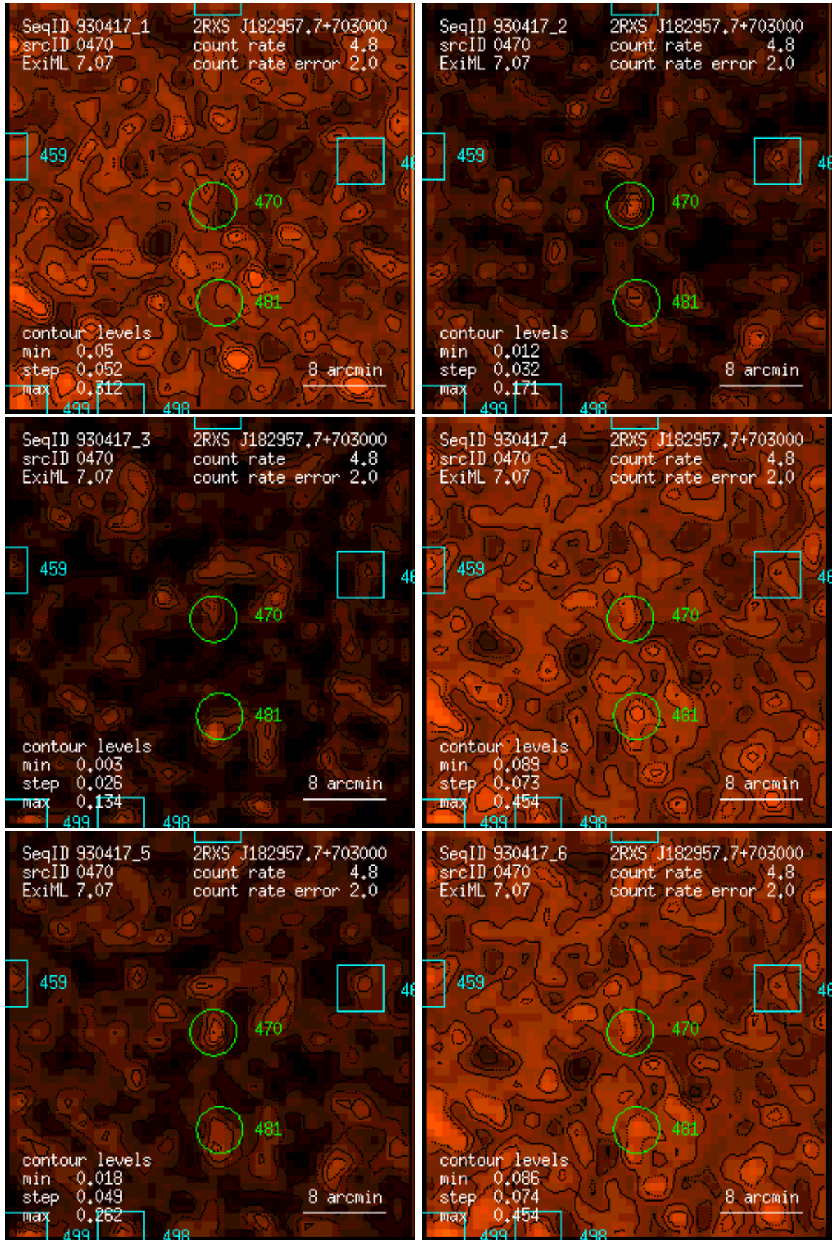
Figure 470: RASS 930417: detection 0470: band rate images, Gaussian filter: (1) PSPC channels 11 – 41, (2) 52 – 90, (3) 91 – 201, (4) 11 – 235, (5) 52 – 201, (6) 11 – 201. Broad band rates in counts/ks. Band rate contour levels in counts/ks/arcmin 2 .
