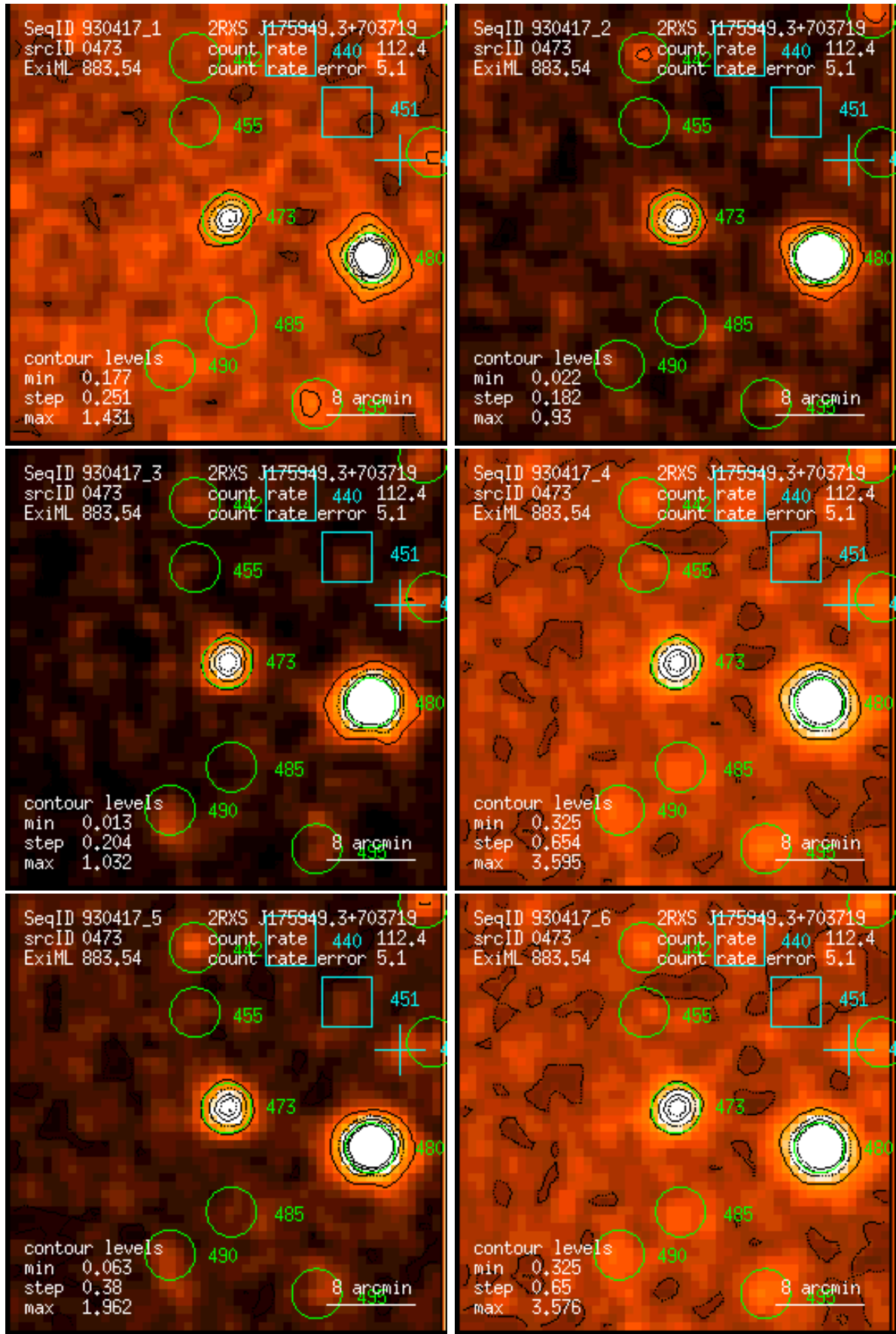
Figure 473: RASS 930417: detection 0473: band rate images, Gaussian filter: (1) PSPC channels 11 – 41, (2) 52 – 90, (3) 91 – 201, (4) 11 – 235, (5) 52 – 201, (6) 11 – 201. Broad band rates in counts/ks. Band rate contour levels in counts/ks/arcmin 2 .
