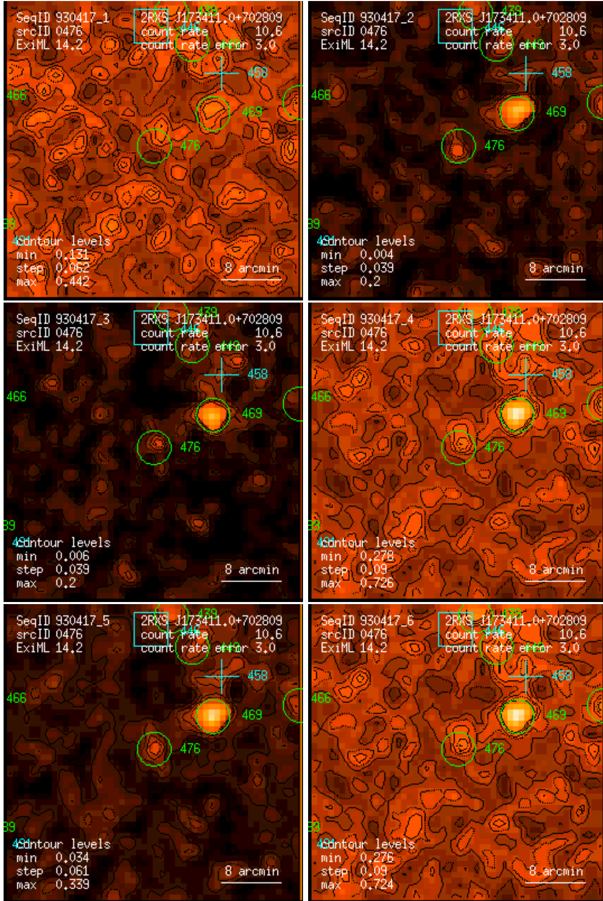
Figure 476: RASS 930417: detection 0476: band rate images, Gaussian filter: (1) PSPC channels 11 – 41, (2) 52 – 90, (3) 91 – 201, (4) 11 – 235, (5) 52 – 201, (6) 11 – 201. Broad band rates in counts/ks. Band rate contour levels in counts/ks/arcmin 2 .
