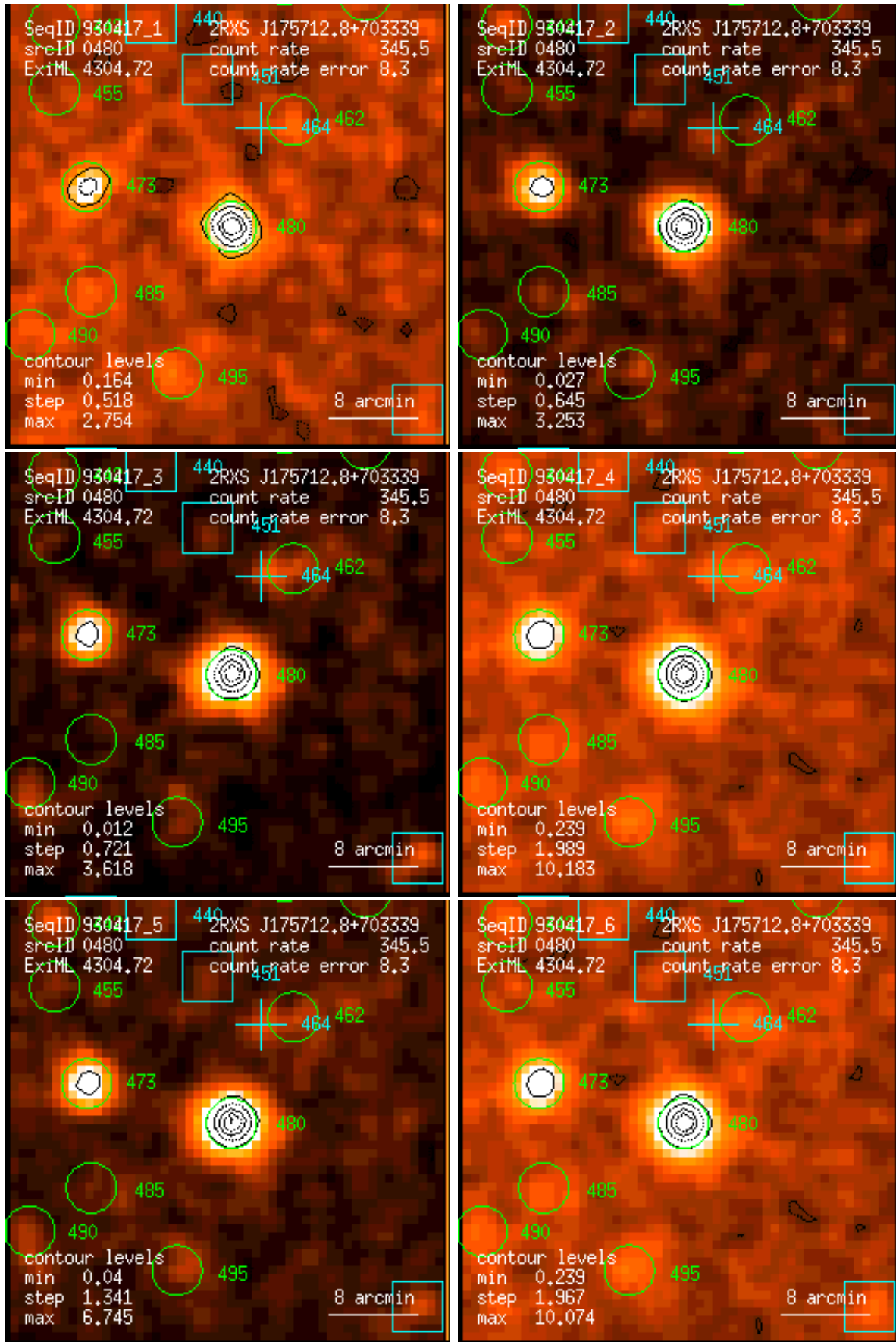
Figure 480: RASS 930417: detection 0480: band rate images, Gaussian filter: (1) PSPC channels 11 – 41, (2) 52 – 90, (3) 91 – 201, (4) 11 – 235, (5) 52 – 201, (6) 11 – 201. Broad band rates in counts/ks. Band rate contour levels in counts/ks/arcmin 2 .
