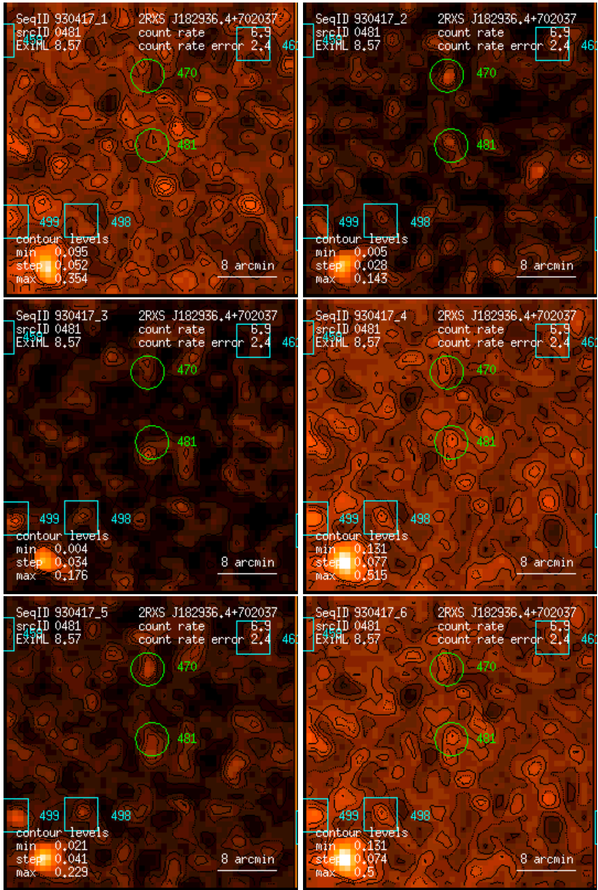
Figure 481: RASS 930417: detection 0481: band rate images, Gaussian filter: (1) PSPC channels 11 – 41, (2) 52 – 90, (3) 91 – 201, (4) 11 – 235, (5) 52 – 201, (6) 11 – 201. Broad band rates in counts/ks. Band rate contour levels in counts/ks/arcmin 2 .
