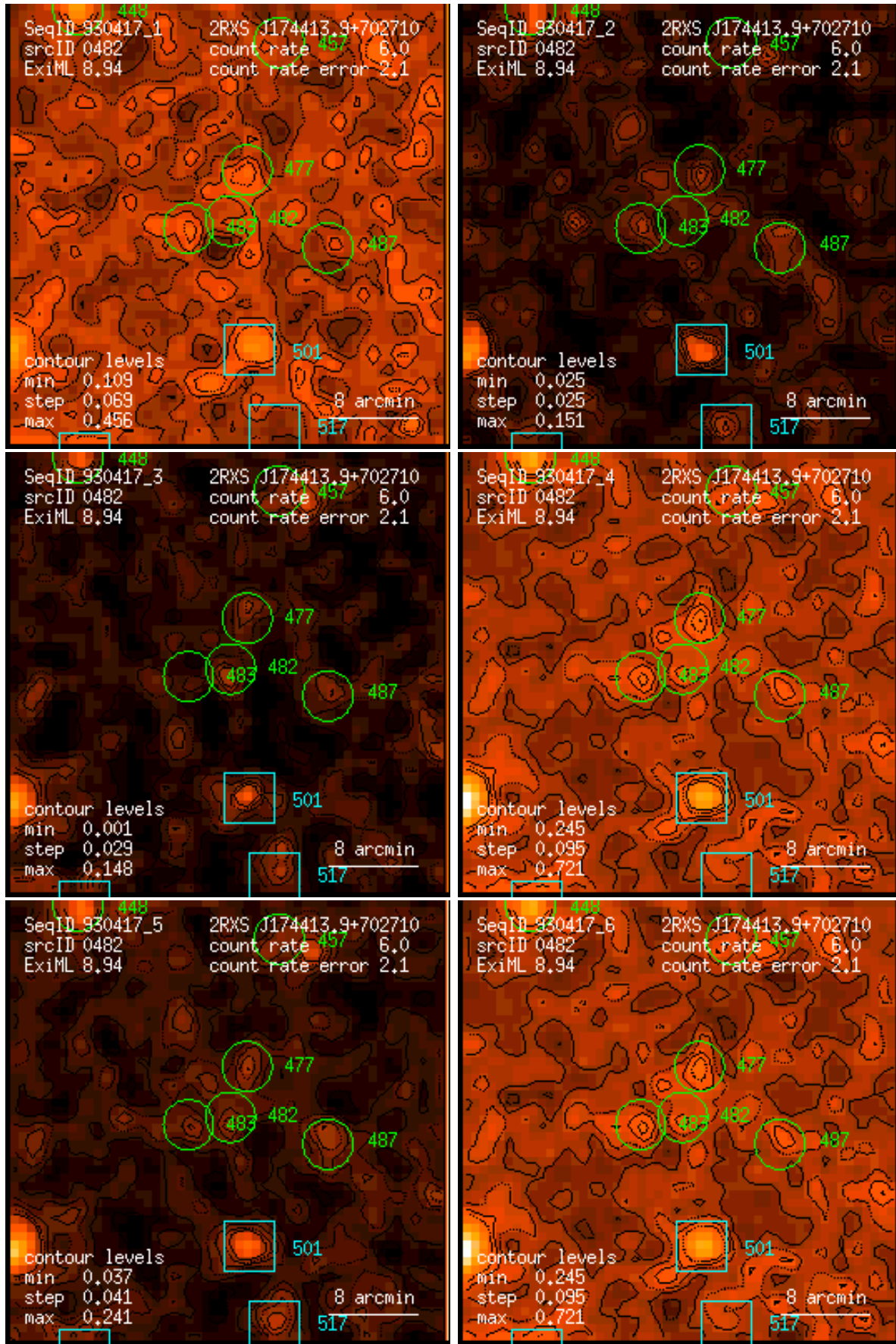
Figure 482: RASS 930417: detection 0482: band rate images, Gaussian filter: (1) PSPC channels 11 – 41, (2) 52 – 90, (3) 91 – 201, (4) 11 – 235, (5) 52 – 201, (6) 11 – 201. Broad band rates in counts/ks. Band rate contour levels in counts/ks/arcmin 2 .
