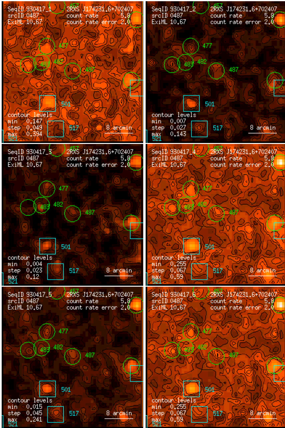
Figure 487: RASS 930417: detection 0487: band rate images, Gaussian filter: (1) PSPC channels 11 – 41, (2) 52 – 90, (3) 91 – 201, (4) 11 – 235, (5) 52 – 201, (6) 11 – 201. Broad band rates in counts/ks. Band rate contour levels in counts/ks/arcmin 2 .
