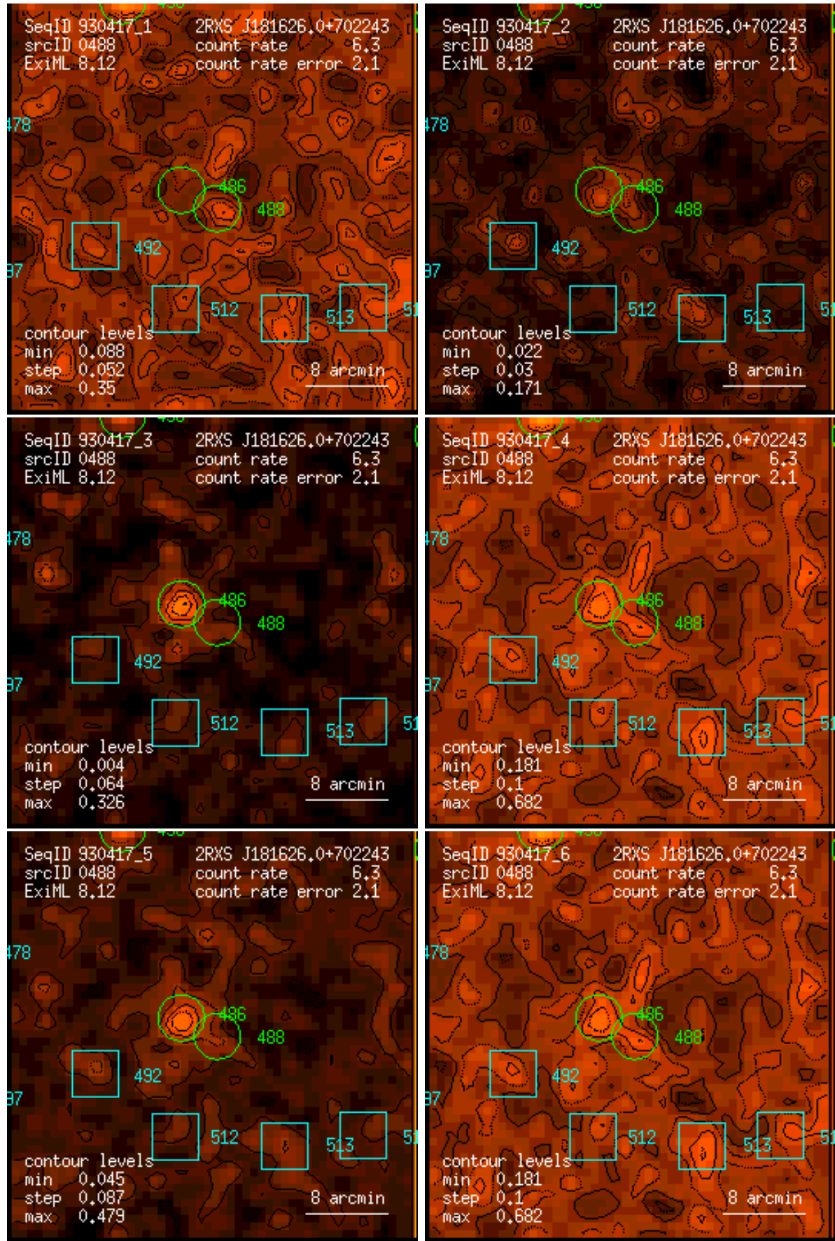
Figure 488: RASS 930417: detection 0488: band rate images, Gaussian filter: (1) PSPC channels 11 – 41, (2) 52 – 90, (3) 91 – 201, (4) 11 – 235, (5) 52 – 201, (6) 11 – 201. Broad band rates in counts/ks. Band rate contour levels in counts/ks/arcmin 2 .
