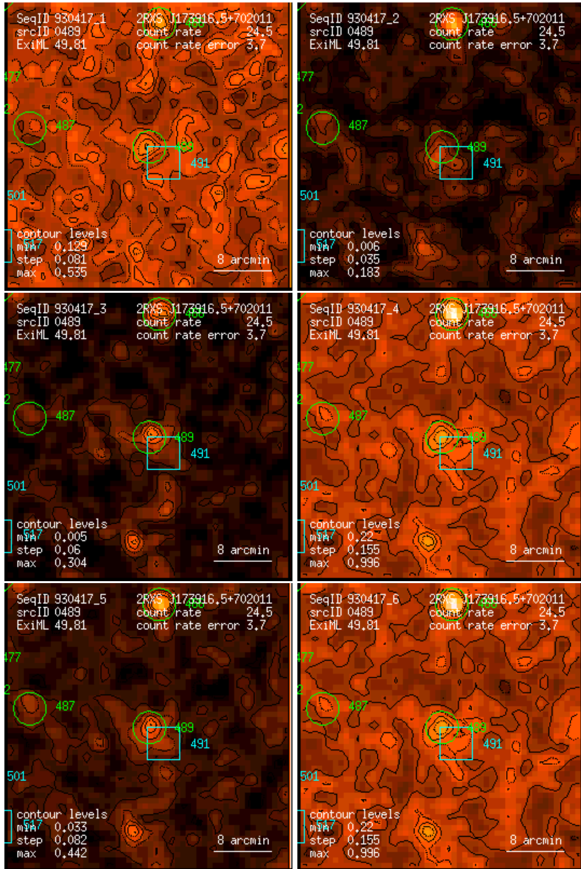
Figure 489: RASS 930417: detection 0489: band rate images, Gaussian filter: (1) PSPC channels 11 – 41, (2) 52 – 90, (3) 91 – 201, (4) 11 – 235, (5) 52 – 201, (6) 11 – 201. Broad band rates in counts/ks. Band rate contour levels in counts/ks/arcmin 2 .
