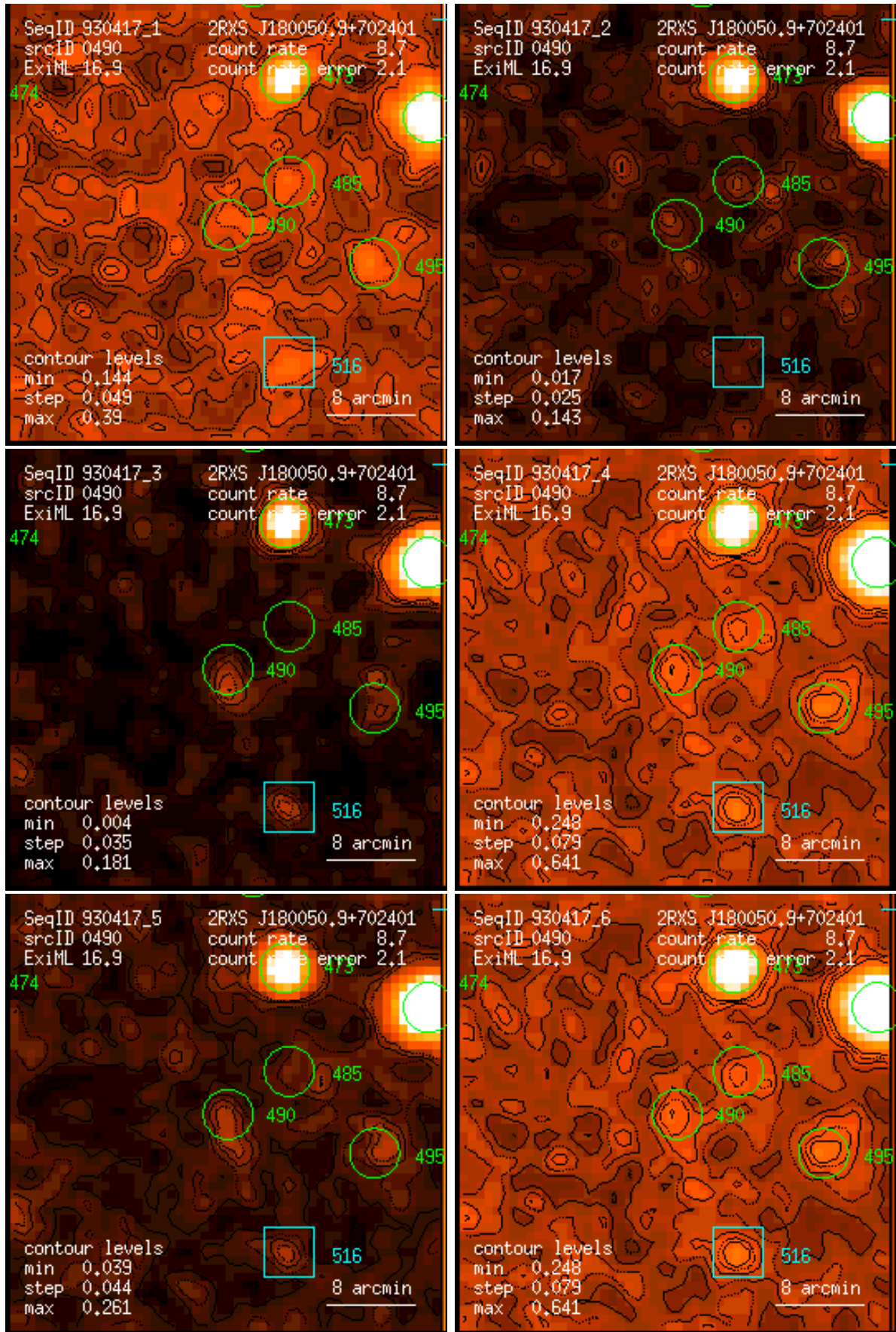
Figure 490: RASS 930417: detection 0490: band rate images, Gaussian filter: (1) PSPC channels 11 – 41, (2) 52 – 90, (3) 91 – 201, (4) 11 – 235, (5) 52 – 201, (6) 11 – 201. Broad band rates in counts/ks. Band rate contour levels in counts/ks/arcmin 2 .
