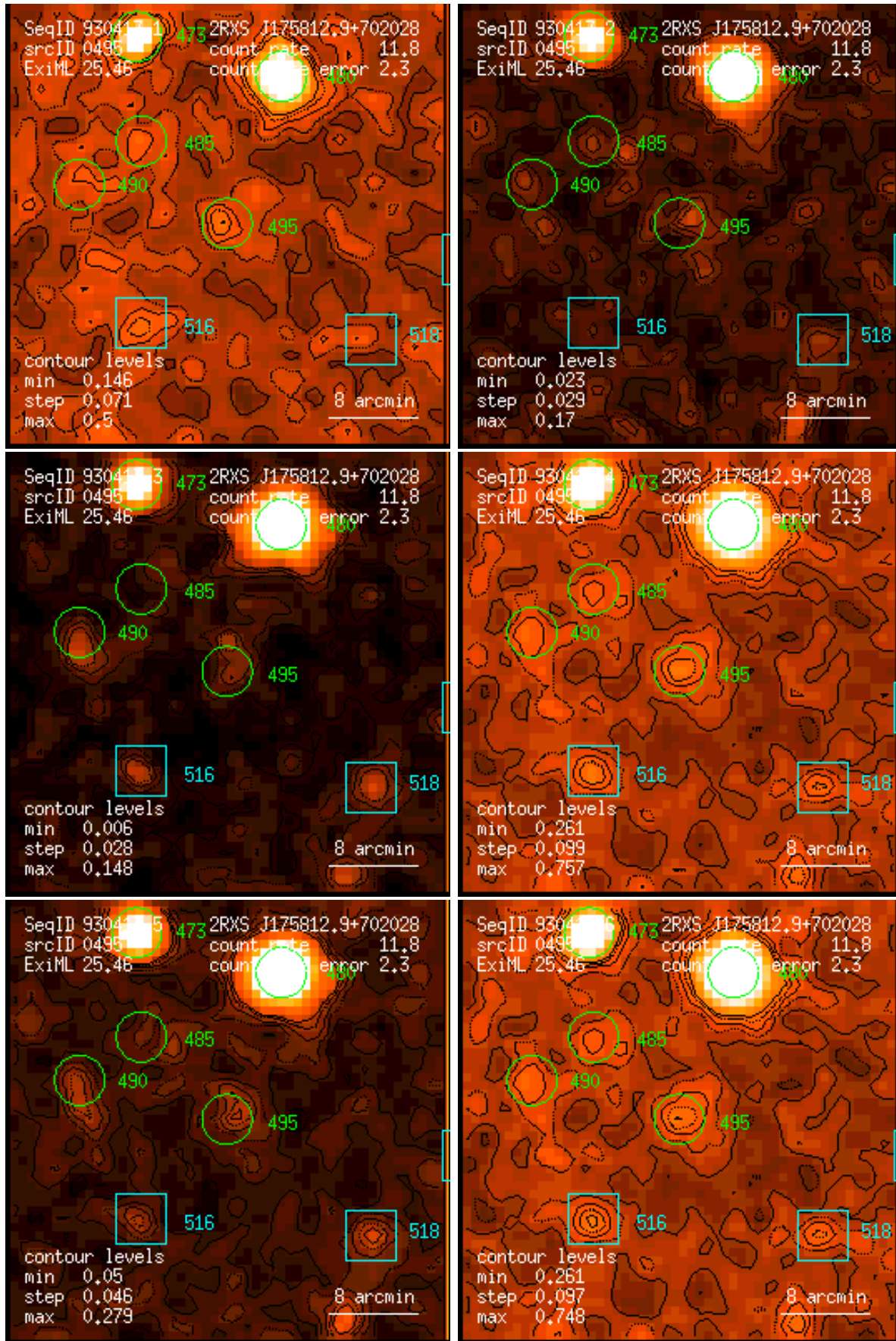
Figure 495: RASS 930417: detection 0495: band rate images, Gaussian filter: (1) PSPC channels 11 – 41, (2) 52 – 90, (3) 91 – 201, (4) 11 – 235, (5) 52 – 201, (6) 11 – 201. Broad band rates in counts/ks. Band rate contour levels in counts/ks/arcmin 2 .
