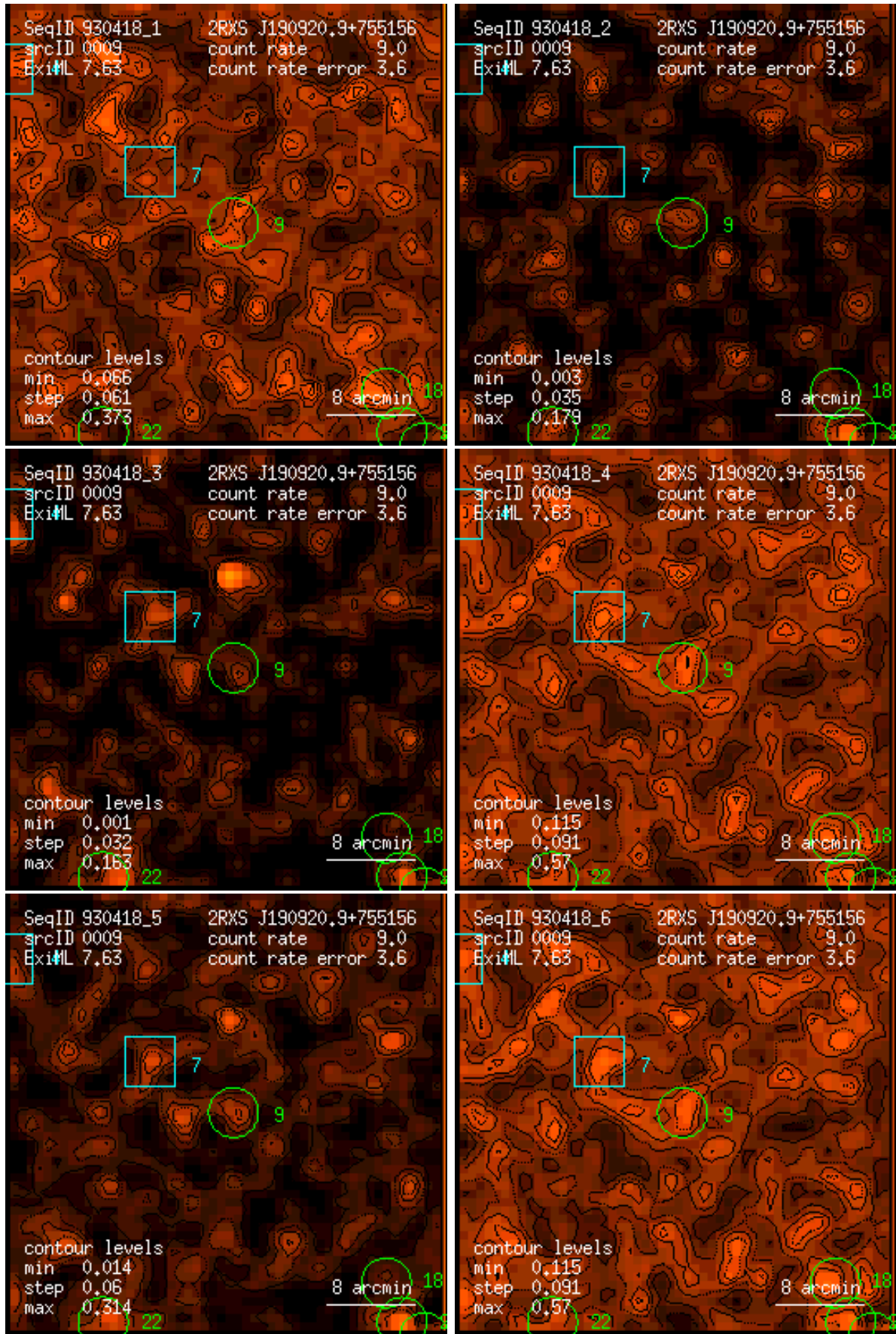
Figure 9: RASS 930418: detection 0009: band rate images, Gaussian filter: (1) PSPC channels 11 – 41, (2) 52 – 90, (3) 91 – 201, (4) 11 – 235, (5) 52 – 201, (6) 11 – 201. Broad band rates in counts/ks. Band rate contour levels in counts/ks/arcmin 2 .
