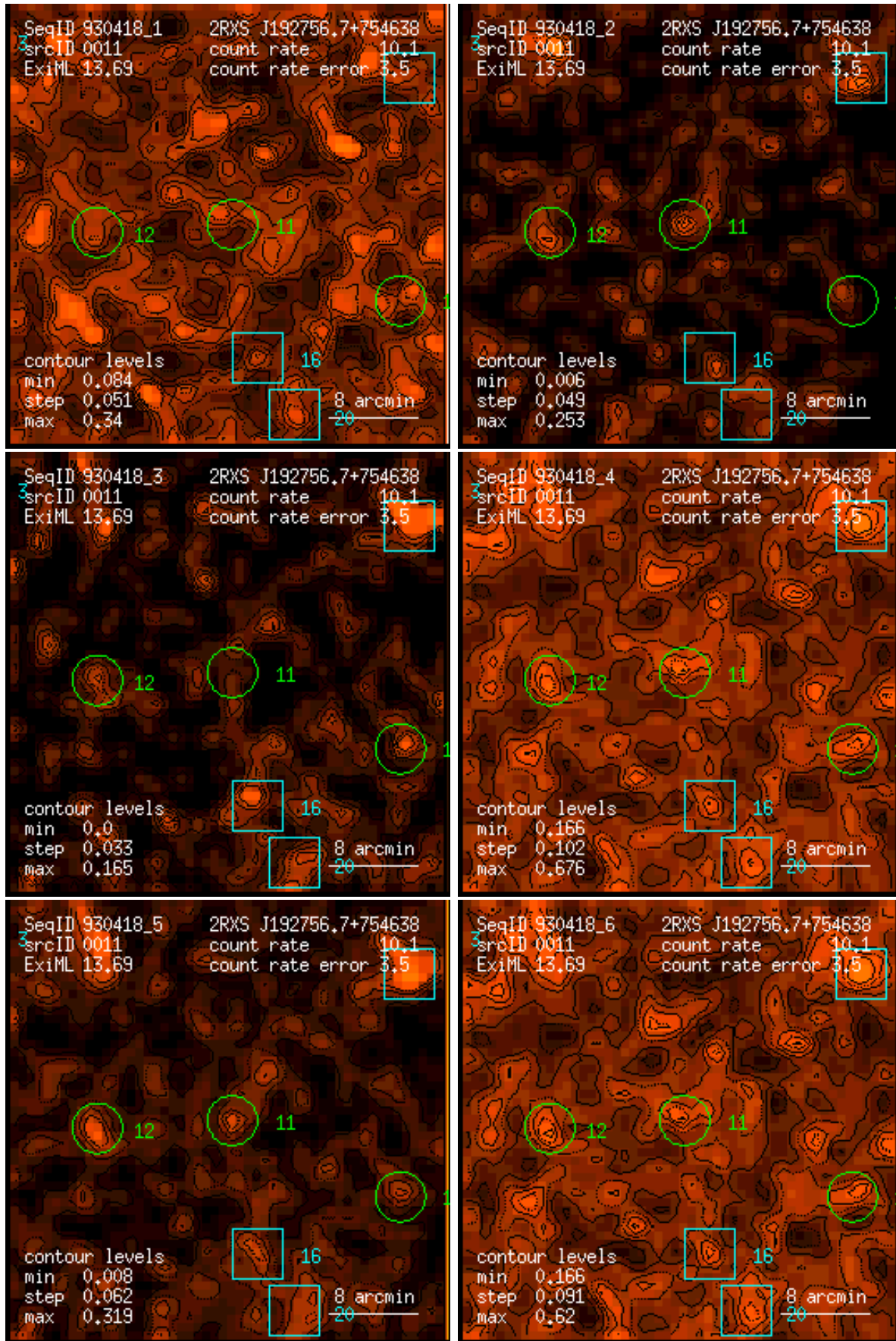
Figure 11: RASS 930418: detection 0011: band rate images, Gaussian filter: (1) PSPC channels 11 – 41, (2) 52 – 90, (3) 91 – 201, (4) 11 – 235, (5) 52 – 201, (6) 11 – 201. Broad band rates in counts/ks. Band rate contour levels in counts/ks/arcmin 2 .
