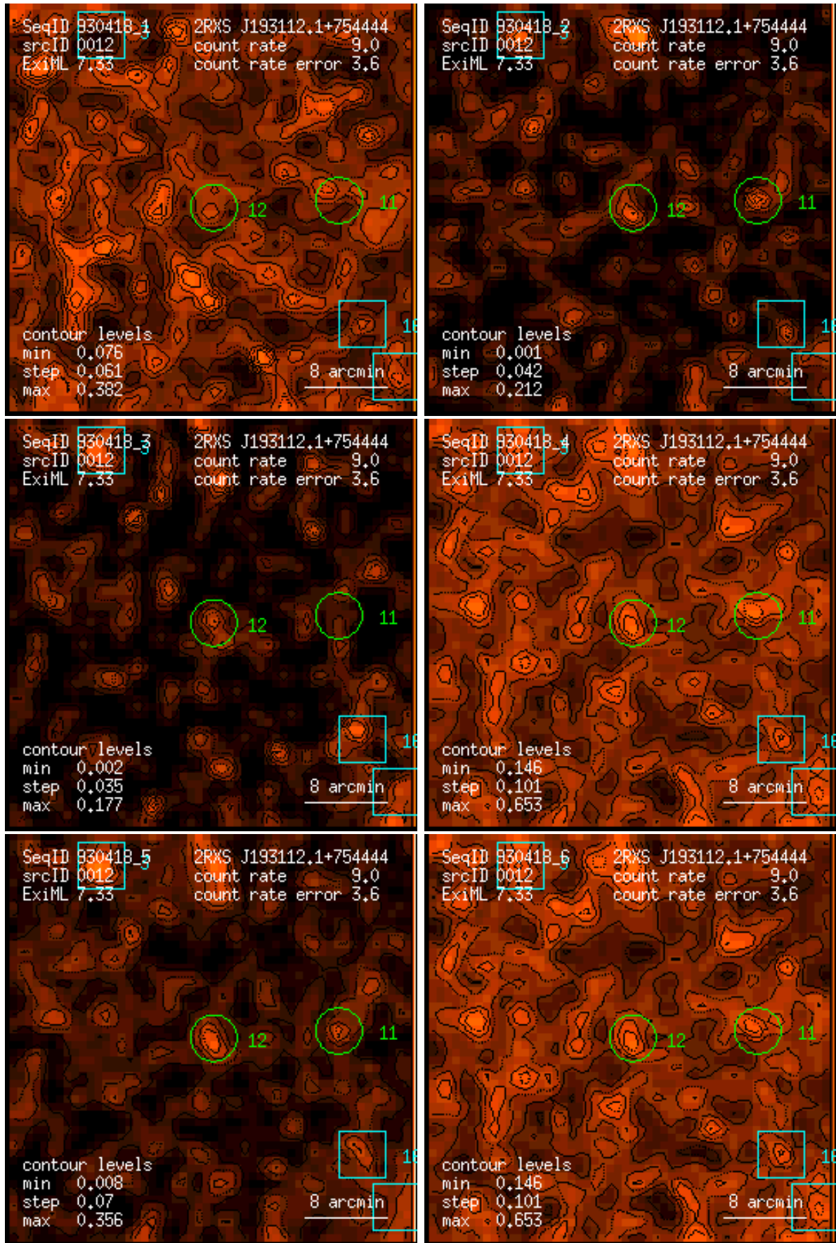
Figure 12: RASS 930418: detection 0012: band rate images, Gaussian filter: (1) PSPC channels 11 – 41, (2) 52 – 90, (3) 91 – 201, (4) 11 – 235, (5) 52 – 201, (6) 11 – 201. Broad band rates in counts/ks. Band rate contour levels in counts/ks/arcmin 2 .
