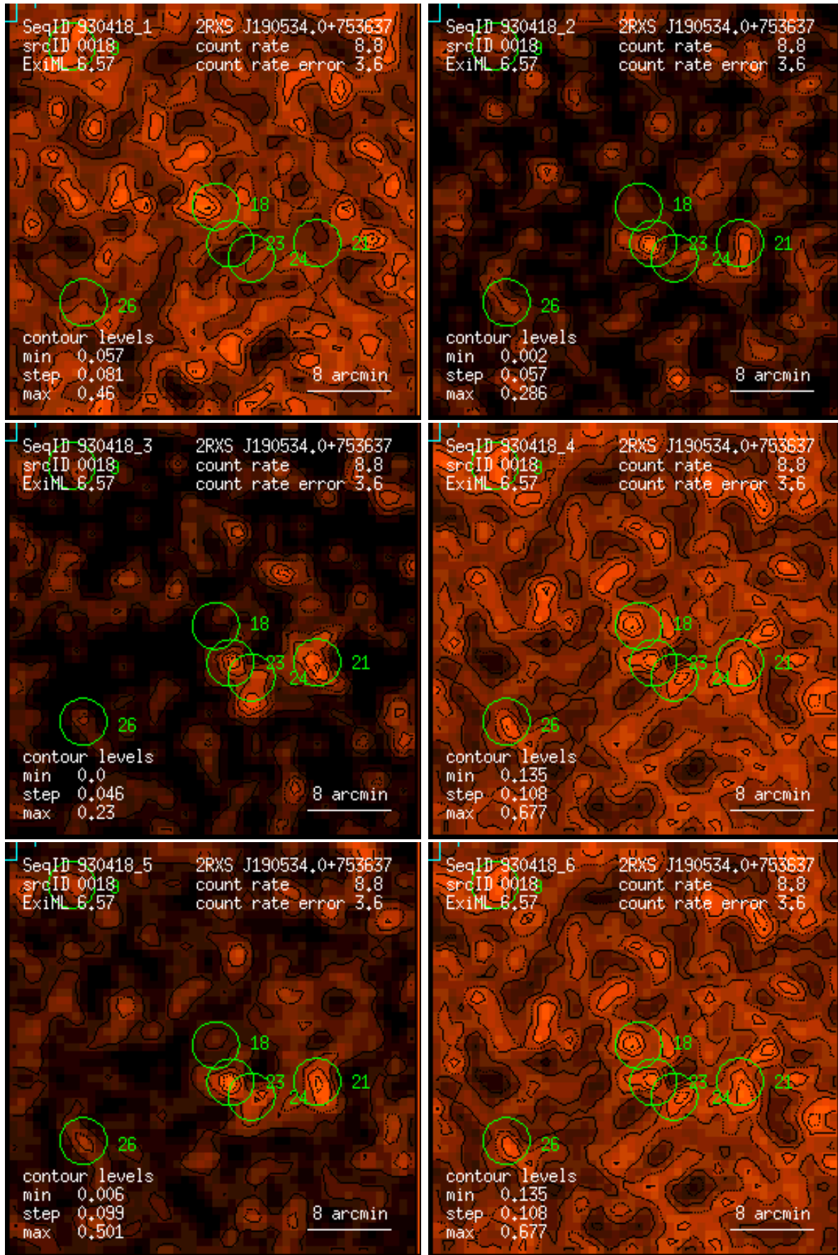
Figure 18: RASS 930418: detection 0018: band rate images, Gaussian filter: (1) PSPC channels 11 – 41, (2) 52 – 90, (3) 91 – 201, (4) 11 – 235, (5) 52 – 201, (6) 11 – 201. Broad band rates in counts/ks. Band rate contour levels in counts/ks/arcmin 2 .
