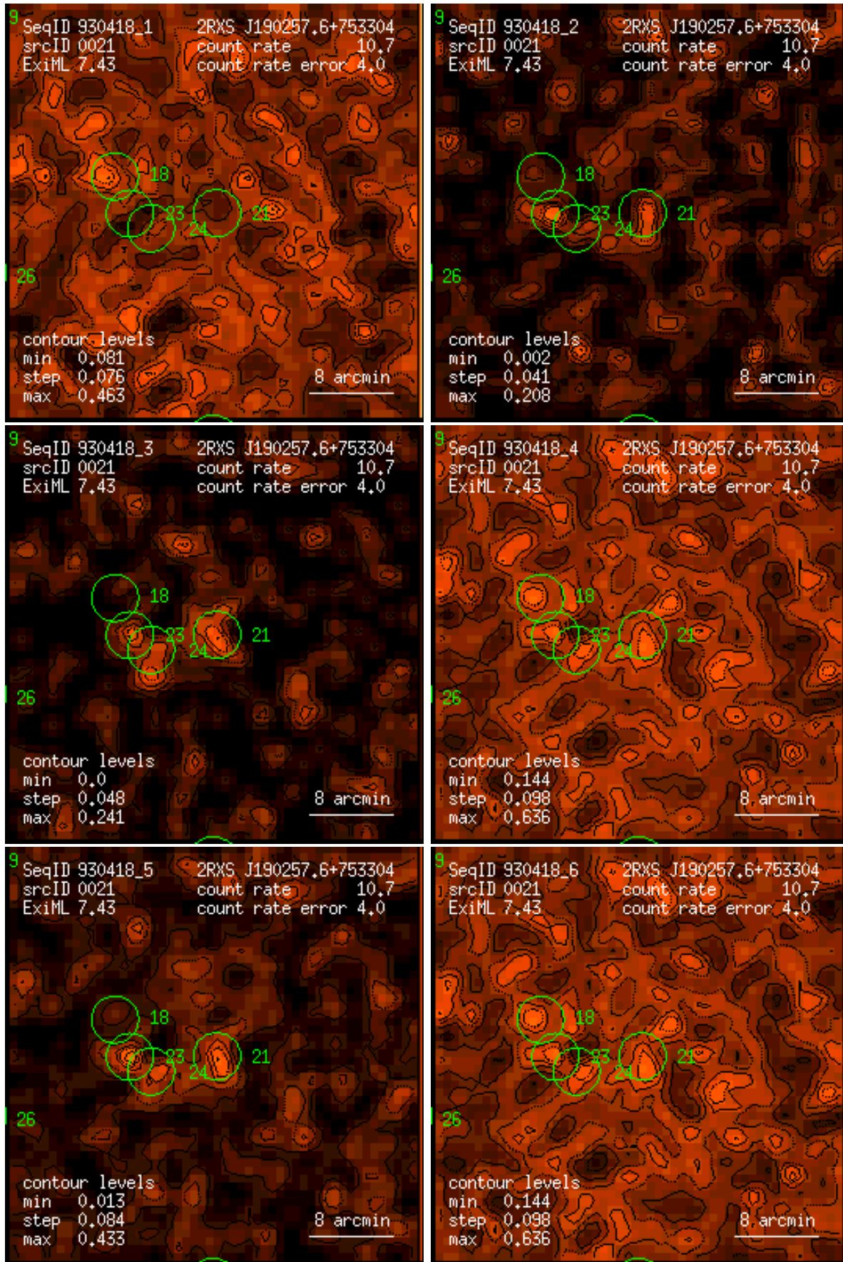
Figure 21: RASS 930418: detection 0021: band rate images, Gaussian filter: (1) PSPC channels 11 – 41, (2) 52 – 90, (3) 91 – 201, (4) 11 – 235, (5) 52 – 201, (6) 11 – 201. Broad band rates in counts/ks. Band rate contour levels in counts/ks/arcmin 2 .
