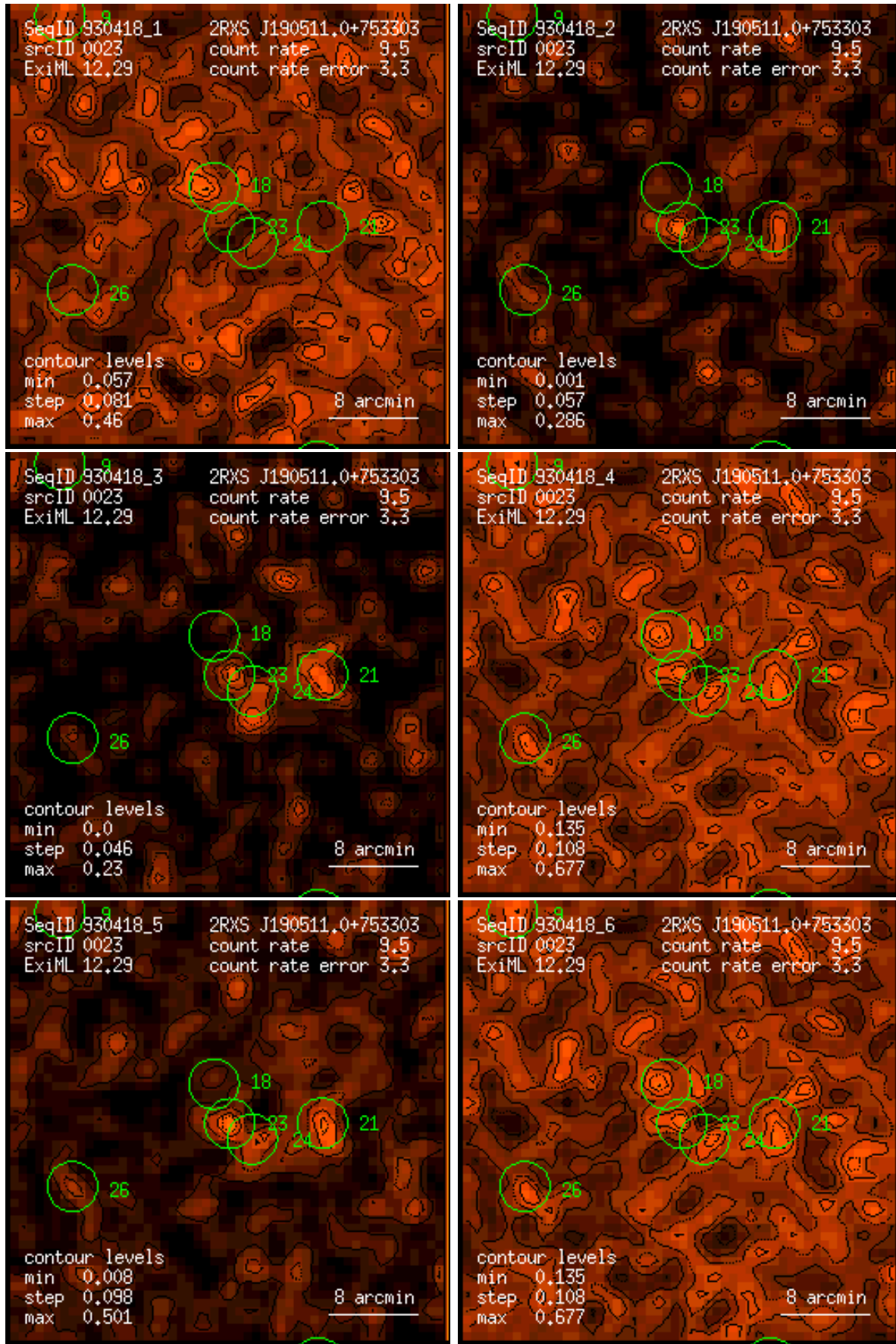
Figure 23: RASS 930418: detection 0023: band rate images, Gaussian filter: (1) PSPC channels 11 – 41, (2) 52 – 90, (3) 91 – 201, (4) 11 – 235, (5) 52 – 201, (6) 11 – 201. Broad band rates in counts/ks. Band rate contour levels in counts/ks/arcmin 2 .
