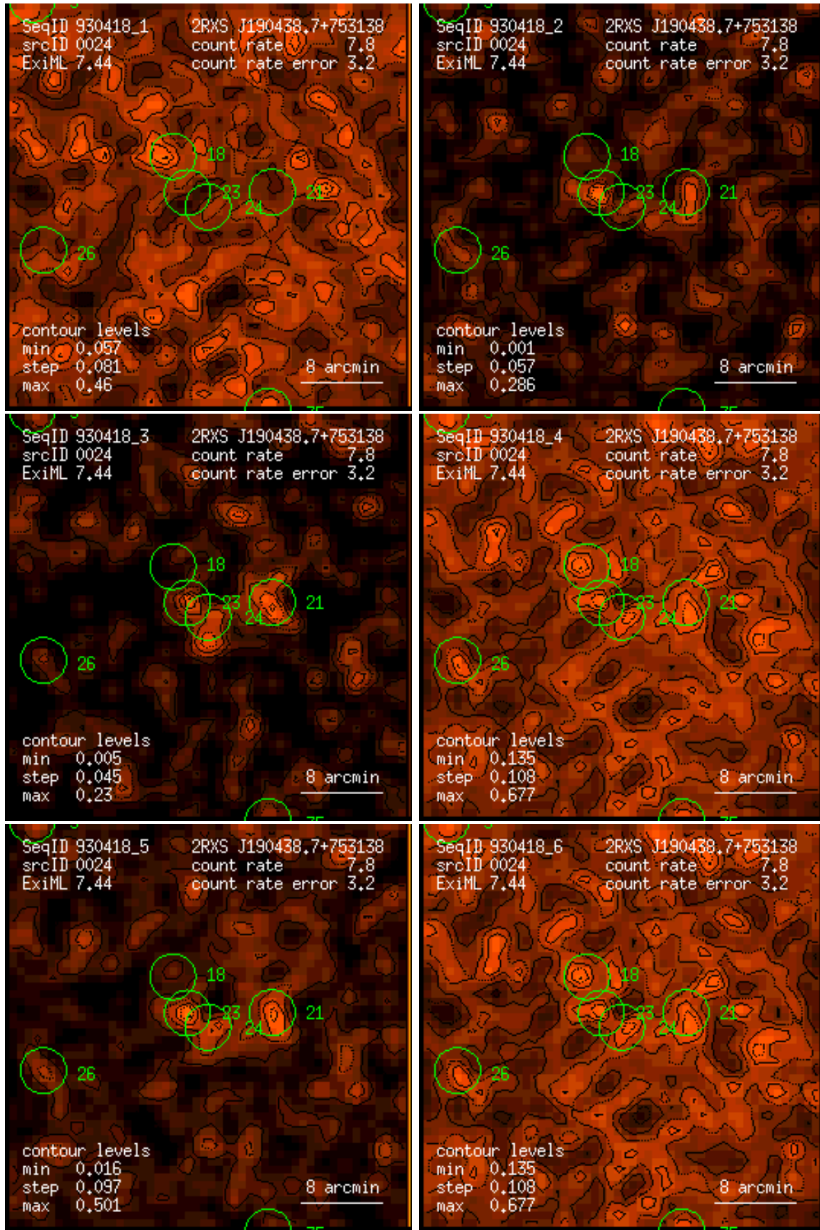
Figure 24: RASS 930418: detection 0024: band rate images, Gaussian filter: (1) PSPC channels 11 – 41, (2) 52 – 90, (3) 91 – 201, (4) 11 – 235, (5) 52 – 201, (6) 11 – 201. Broad band rates in counts/ks. Band rate contour levels in counts/ks/arcmin 2 .
