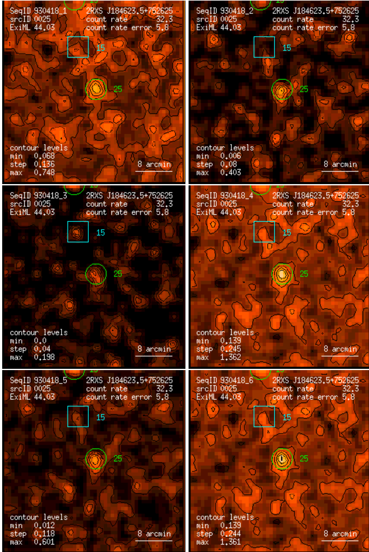
Figure 25: RASS 930418: detection 0025: band rate images, Gaussian filter: (1) PSPC channels 11 – 41, (2) 52 – 90, (3) 91 – 201, (4) 11 – 235, (5) 52 – 201, (6) 11 – 201. Broad band rates in counts/ks. Band rate contour levels in counts/ks/arcmin 2 .
