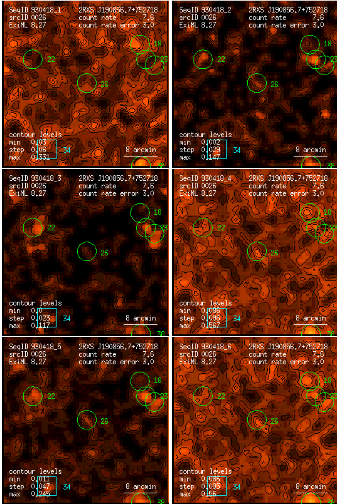
Figure 26: RASS 930418: detection 0026: band rate images, Gaussian filter: (1) PSPC channels 11 – 41, (2) 52 – 90, (3) 91 – 201, (4) 11 – 235, (5) 52 – 201, (6) 11 – 201. Broad band rates in counts/ks. Band rate contour levels in counts/ks/arcmin 2 .
