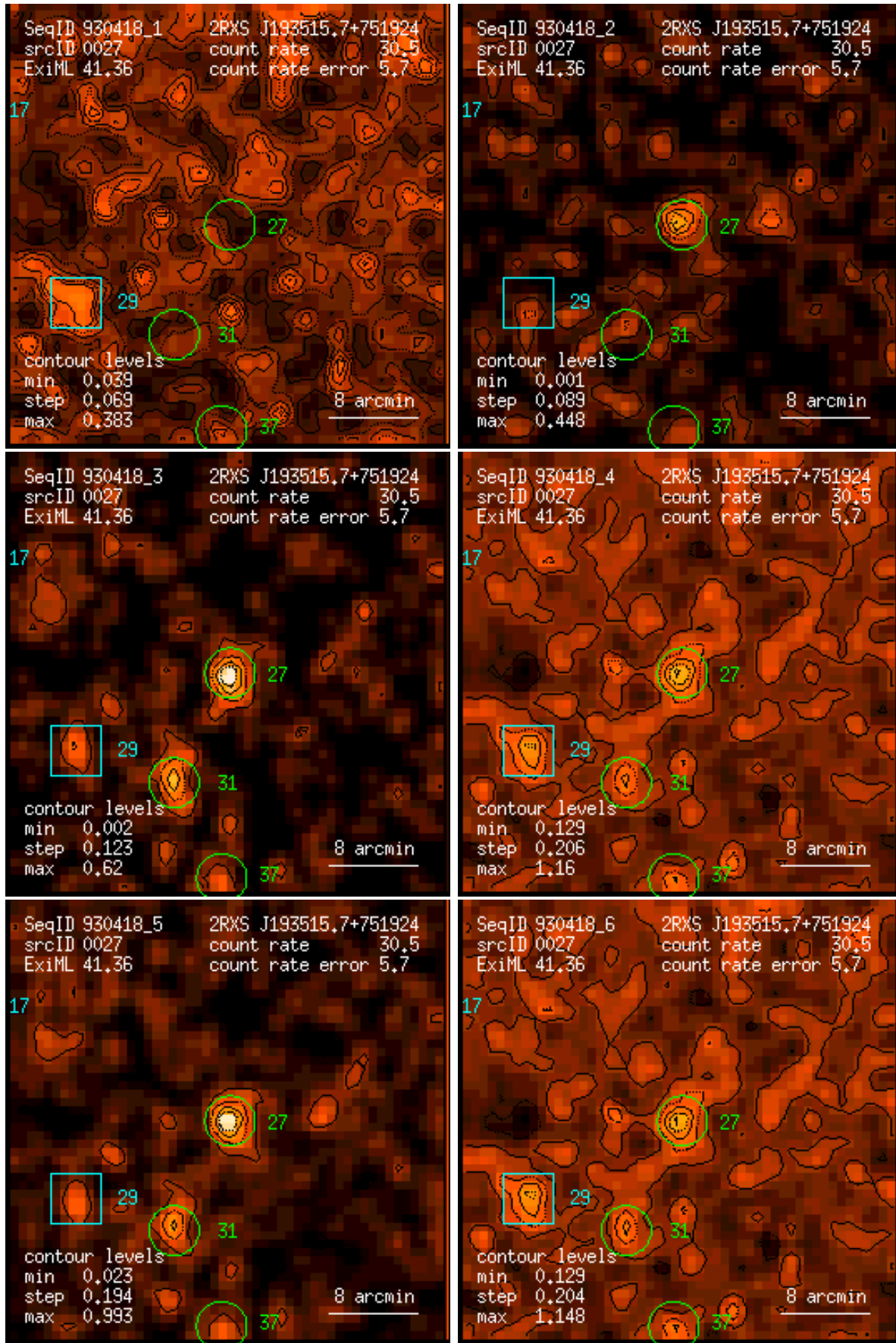
Figure 27: RASS 930418: detection 0027: band rate images, Gaussian filter: (1) PSPC channels 11 – 41, (2) 52 – 90, (3) 91 – 201, (4) 11 – 235, (5) 52 – 201, (6) 11 – 201. Broad band rates in counts/ks. Band rate contour levels in counts/ks/arcmin 2 .
