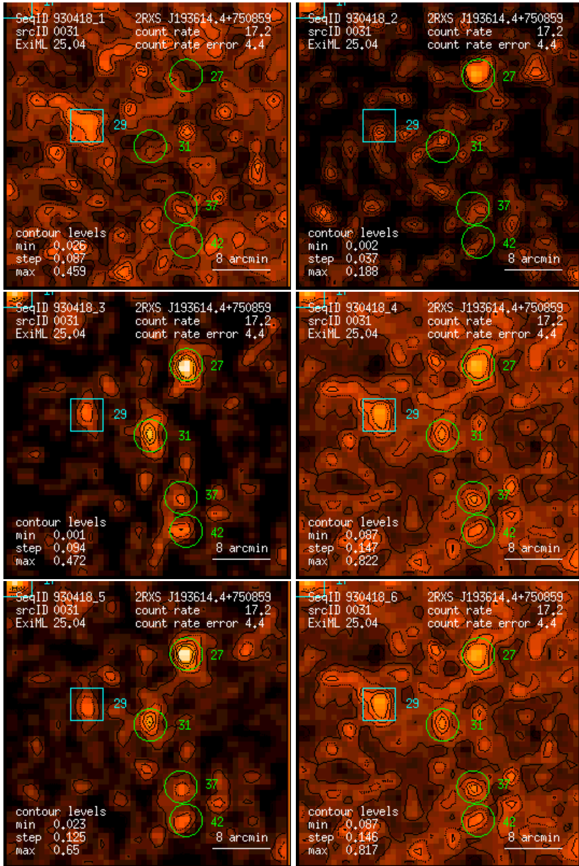
Figure 31: RASS 930418: detection 0031: band rate images, Gaussian filter: (1) PSPC channels 11 – 41, (2) 52 – 90, (3) 91 – 201, (4) 11 – 235, (5) 52 – 201, (6) 11 – 201. Broad band rates in counts/ks. Band rate contour levels in counts/ks/arcmin 2 .
