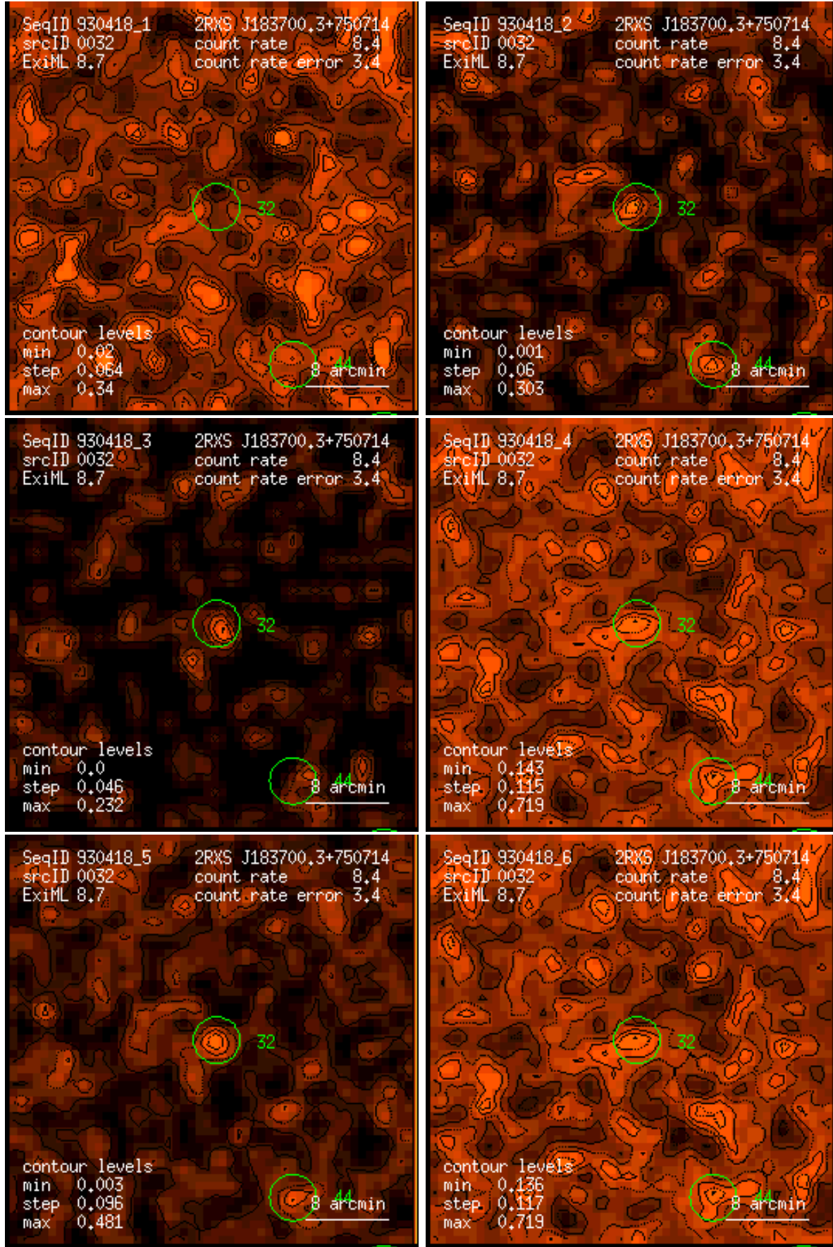
Figure 32: RASS 930418: detection 0032: band rate images, Gaussian filter: (1) PSPC channels 11 – 41, (2) 52 – 90, (3) 91 – 201, (4) 11 – 235, (5) 52 – 201, (6) 11 – 201. Broad band rates in counts/ks. Band rate contour levels in counts/ks/arcmin 2 .
