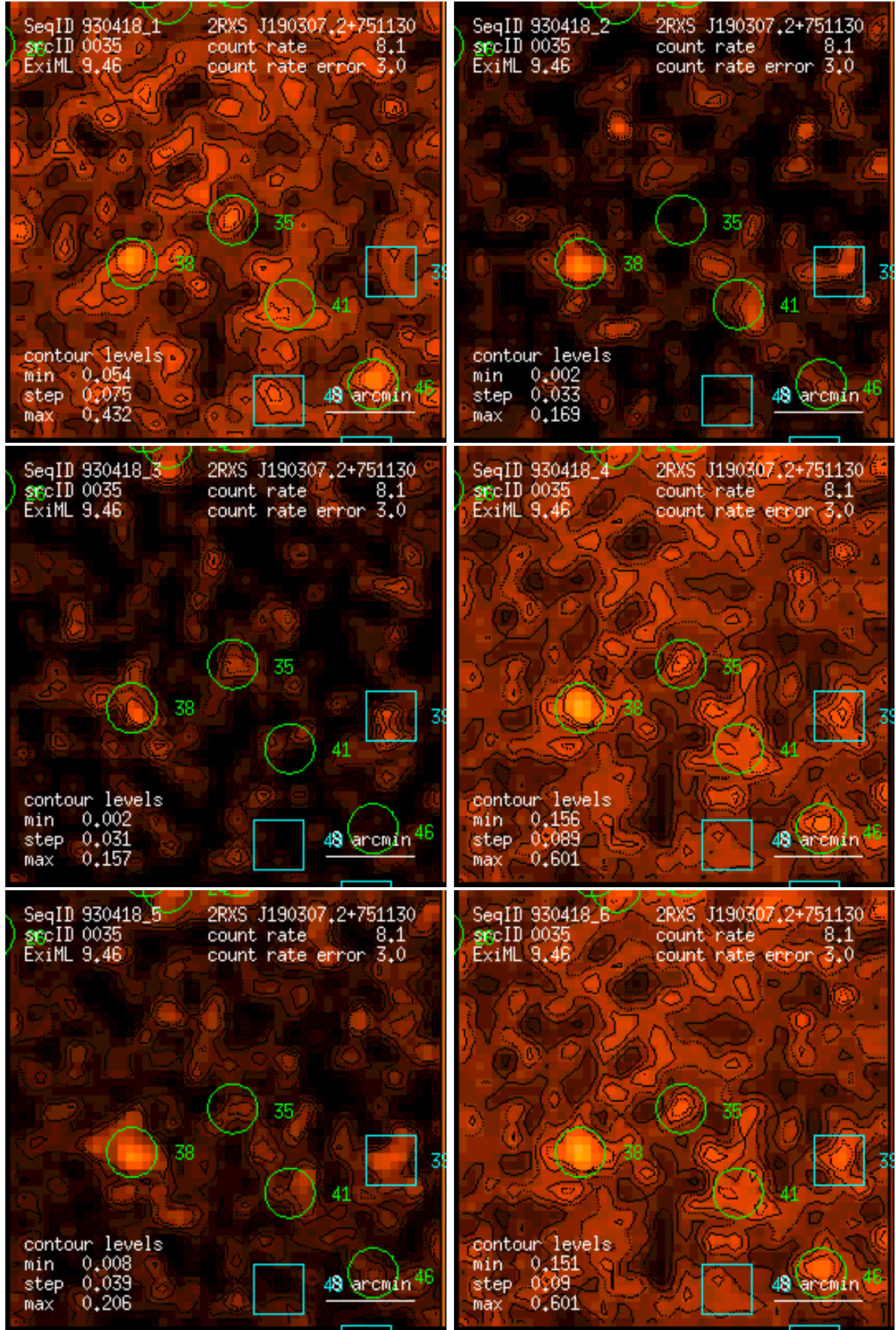
Figure 35: RASS 930418: detection 0035: band rate images, Gaussian filter: (1) PSPC channels 11 – 41, (2) 52 – 90, (3) 91 – 201, (4) 11 – 235, (5) 52 – 201, (6) 11 – 201. Broad band rates in counts/ks. Band rate contour levels in counts/ks/arcmin 2 .
