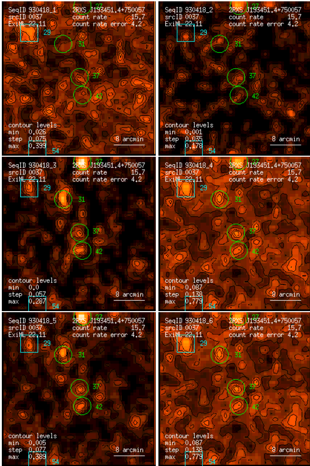
Figure 37: RASS 930418: detection 0037: band rate images, Gaussian filter: (1) PSPC channels 11 – 41, (2) 52 – 90, (3) 91 – 201, (4) 11 – 235, (5) 52 – 201, (6) 11 – 201. Broad band rates in counts/ks. Band rate contour levels in counts/ks/arcmin 2 .
