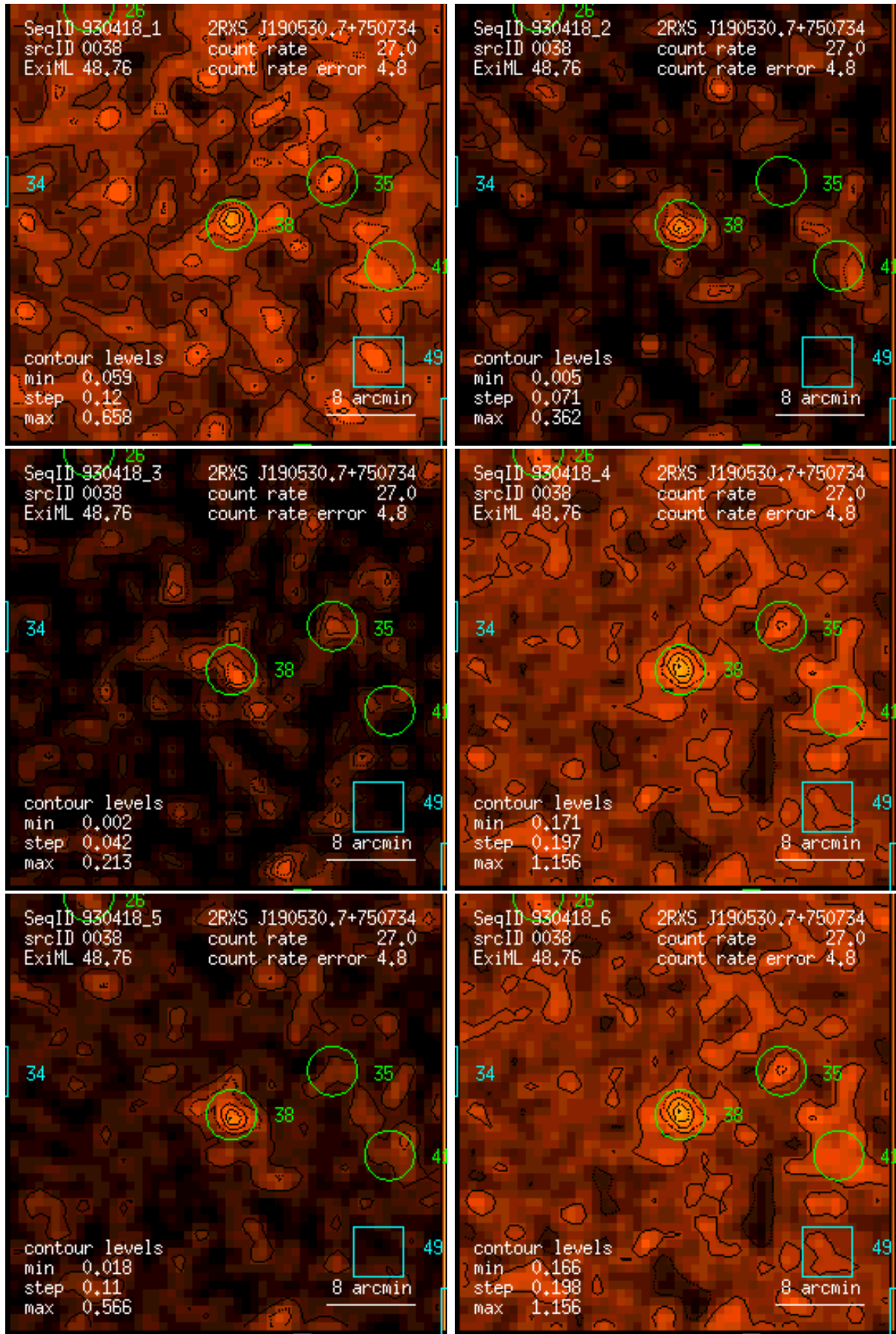
Figure 38: RASS 930418: detection 0038: band rate images, Gaussian filter: (1) PSPC channels 11 – 41, (2) 52 – 90, (3) 91 – 201, (4) 11 – 235, (5) 52 – 201, (6) 11 – 201. Broad band rates in counts/ks. Band rate contour levels in counts/ks/arcmin 2 .
