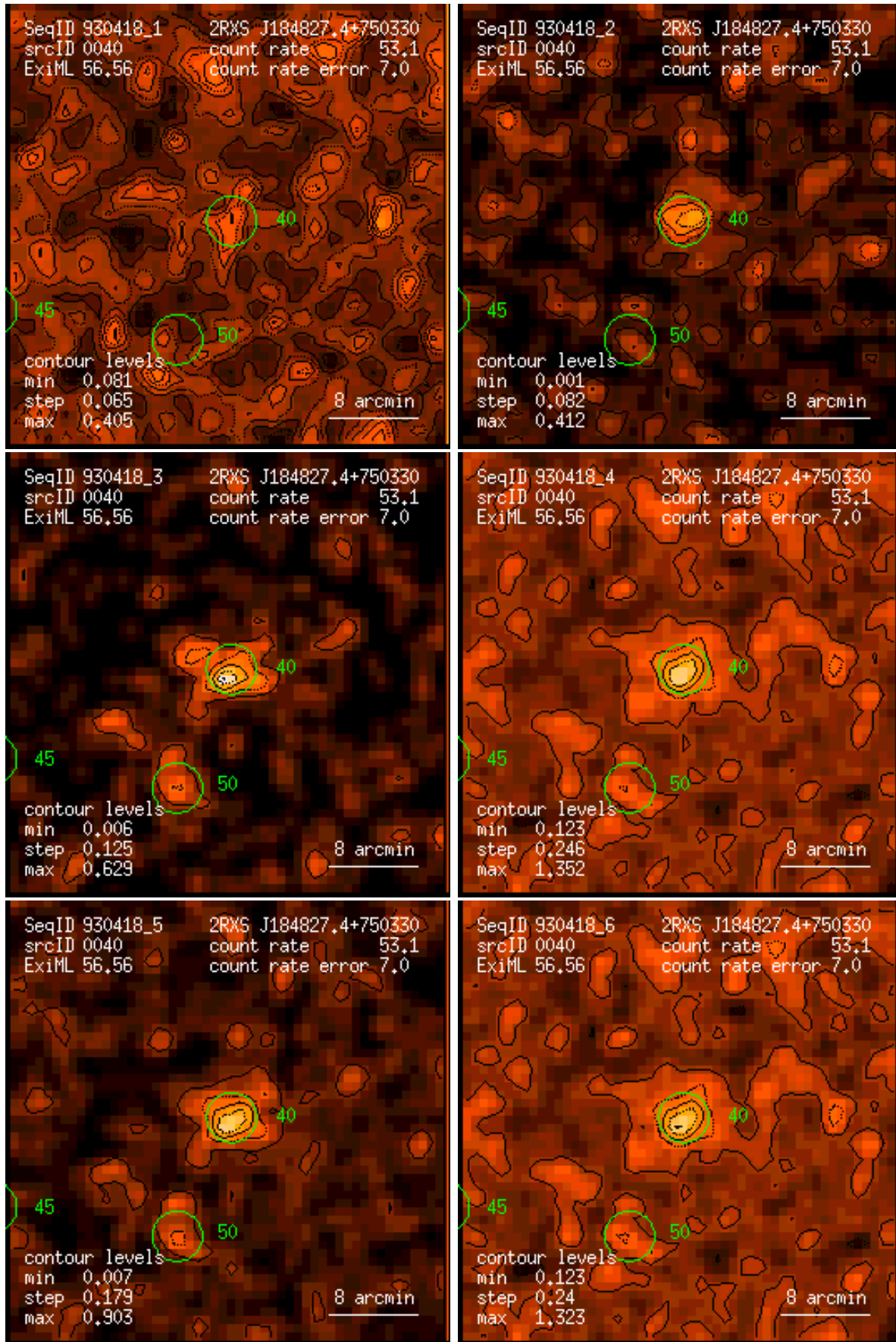
Figure 40: RASS 930418: detection 0040: band rate images, Gaussian filter: (1) PSPC channels 11 – 41, (2) 52 – 90, (3) 91 – 201, (4) 11 – 235, (5) 52 – 201, (6) 11 – 201. Broad band rates in counts/ks. Band rate contour levels in counts/ks/arcmin 2 .
