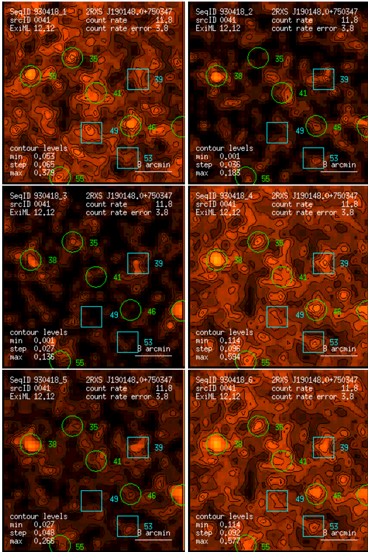
Figure 41: RASS 930418: detection 0041: band rate images, Gaussian filter: (1) PSPC channels 11 – 41, (2) 52 – 90, (3) 91 – 201, (4) 11 – 235, (5) 52 – 201, (6) 11 – 201. Broad band rates in counts/ks. Band rate contour levels in counts/ks/arcmin 2 .
