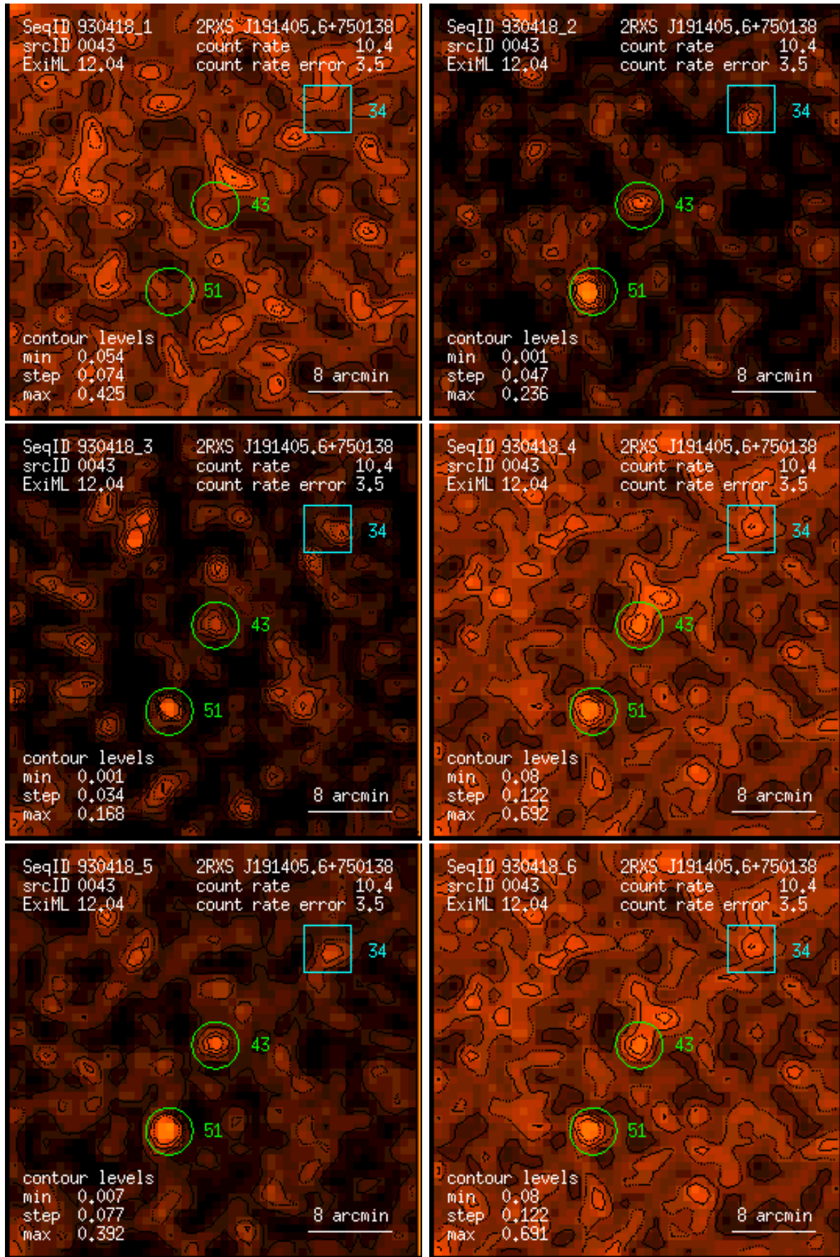
Figure 43: RASS 930418: detection 0043: band rate images, Gaussian filter: (1) PSPC channels 11 – 41, (2) 52 – 90, (3) 91 – 201, (4) 11 – 235, (5) 52 – 201, (6) 11 – 201. Broad band rates in counts/ks. Band rate contour levels in counts/ks/arcmin 2 .
