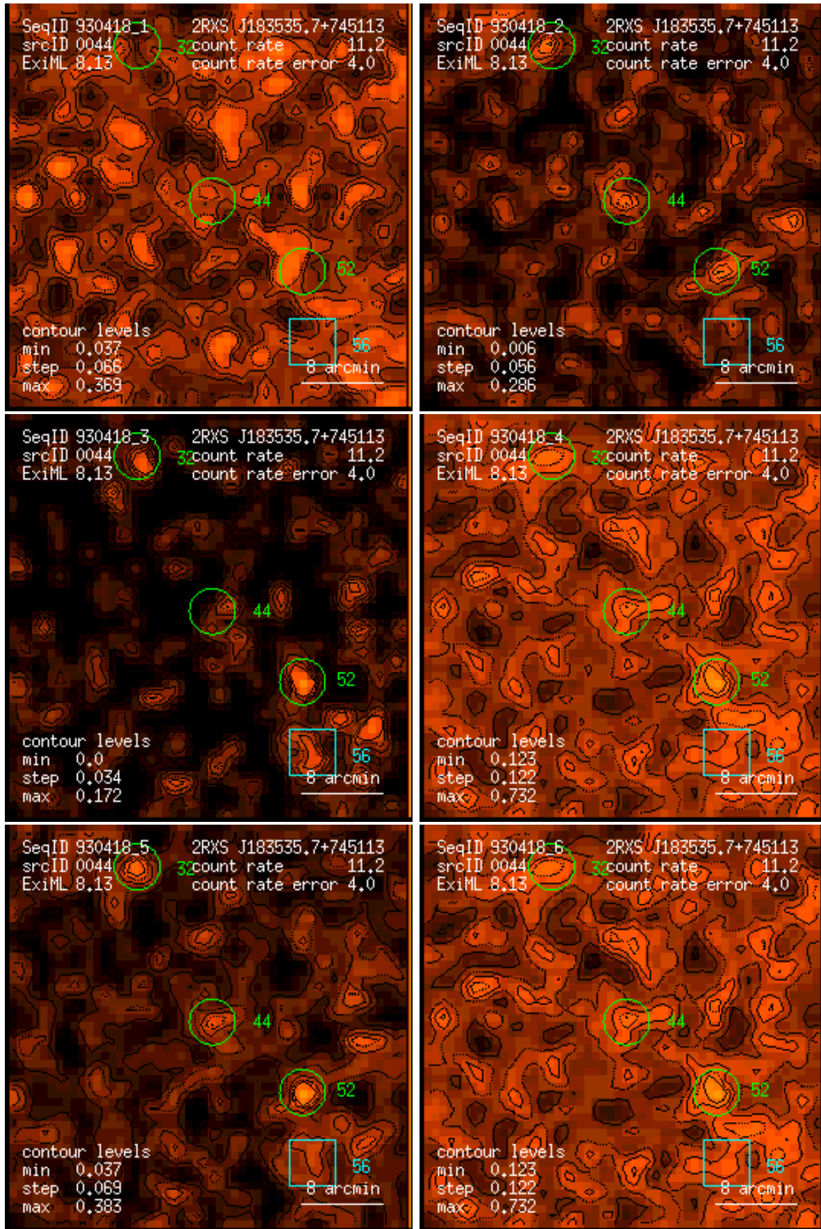
Figure 44: RASS 930418: detection 0044: band rate images, Gaussian filter: (1) PSPC channels 11 – 41, (2) 52 – 90, (3) 91 – 201, (4) 11 – 235, (5) 52 – 201, (6) 11 – 201. Broad band rates in counts/ks. Band rate contour levels in counts/ks/arcmin 2 .
