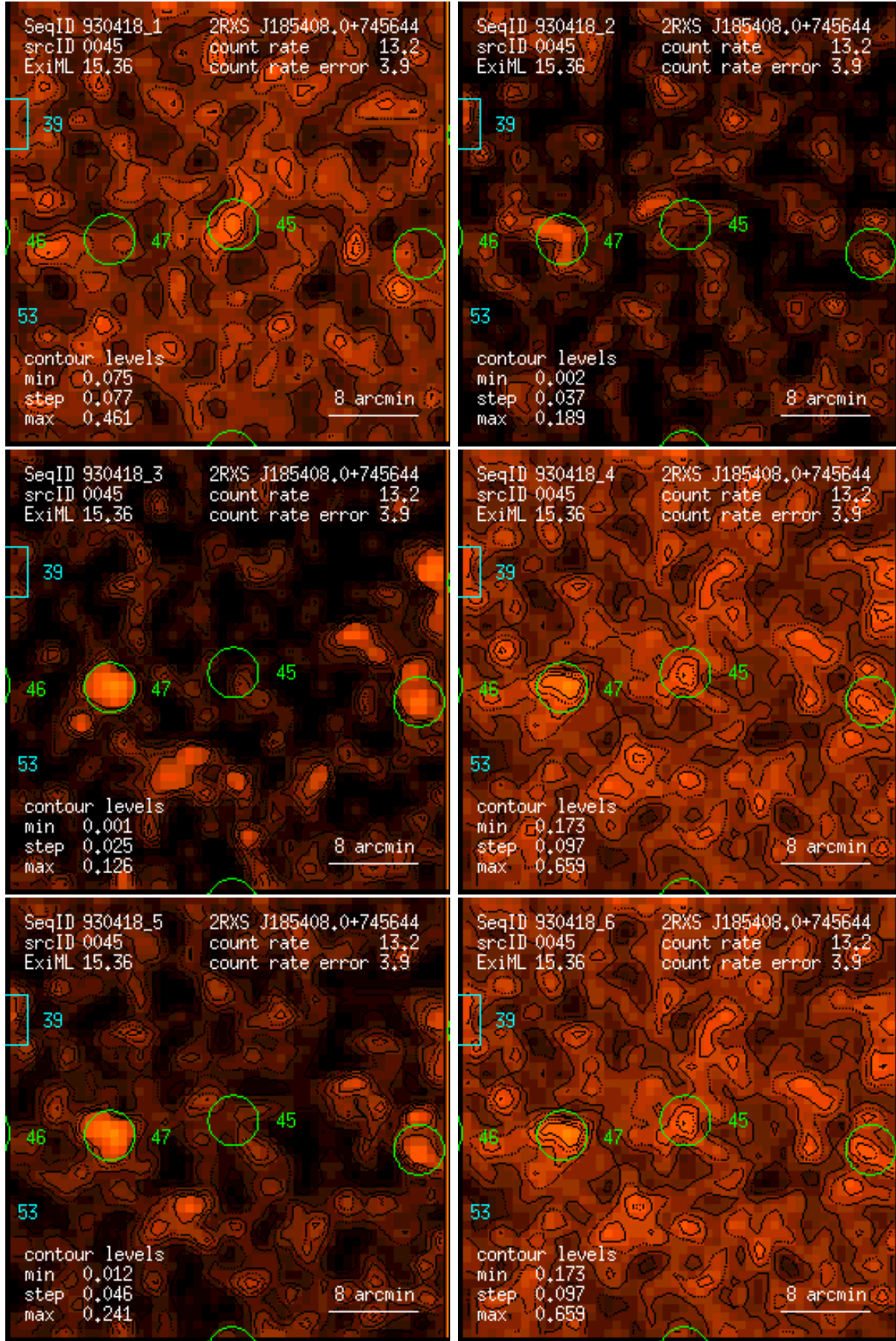
Figure 45: RASS 930418: detection 0045: band rate images, Gaussian filter: (1) PSPC channels 11 – 41, (2) 52 – 90, (3) 91 – 201, (4) 11 – 235, (5) 52 – 201, (6) 11 – 201. Broad band rates in counts/ks. Band rate contour levels in counts/ks/arcmin 2 .
