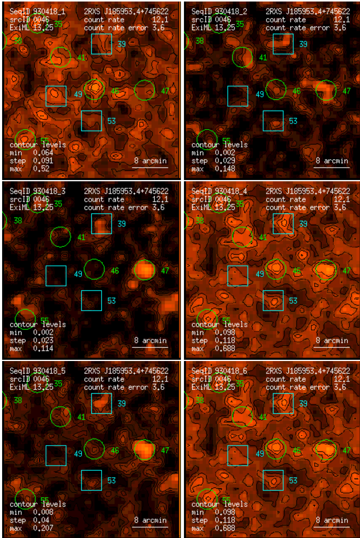
Figure 46: RASS 930418: detection 0046: band rate images, Gaussian filter: (1) PSPC channels 11 – 41, (2) 52 – 90, (3) 91 – 201, (4) 11 – 235, (5) 52 – 201, (6) 11 – 201. Broad band rates in counts/ks. Band rate contour levels in counts/ks/arcmin 2 .
