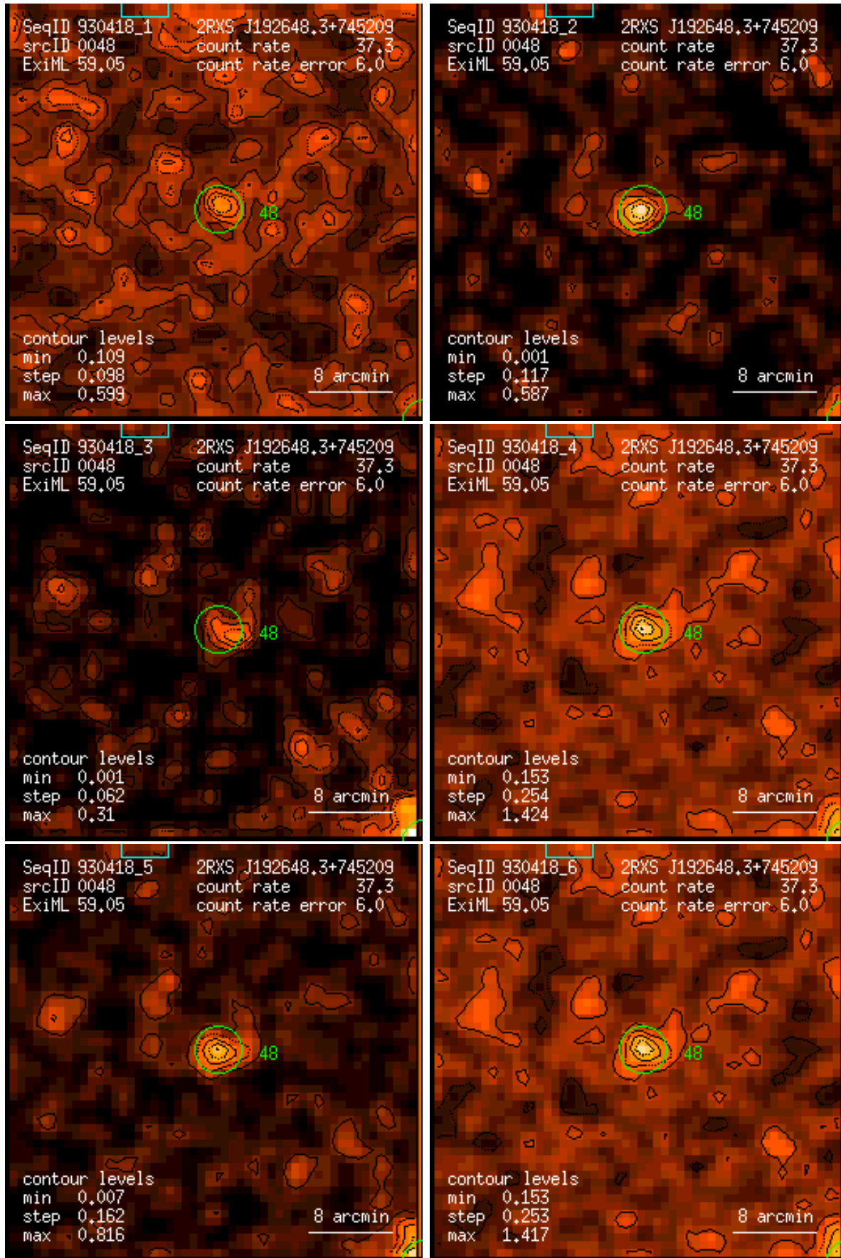
Figure 48: RASS 930418: detection 0048: band rate images, Gaussian filter: (1) PSPC channels 11 – 41, (2) 52 – 90, (3) 91 – 201, (4) 11 – 235, (5) 52 – 201, (6) 11 – 201. Broad band rates in counts/ks. Band rate contour levels in counts/ks/arcmin 2 .
