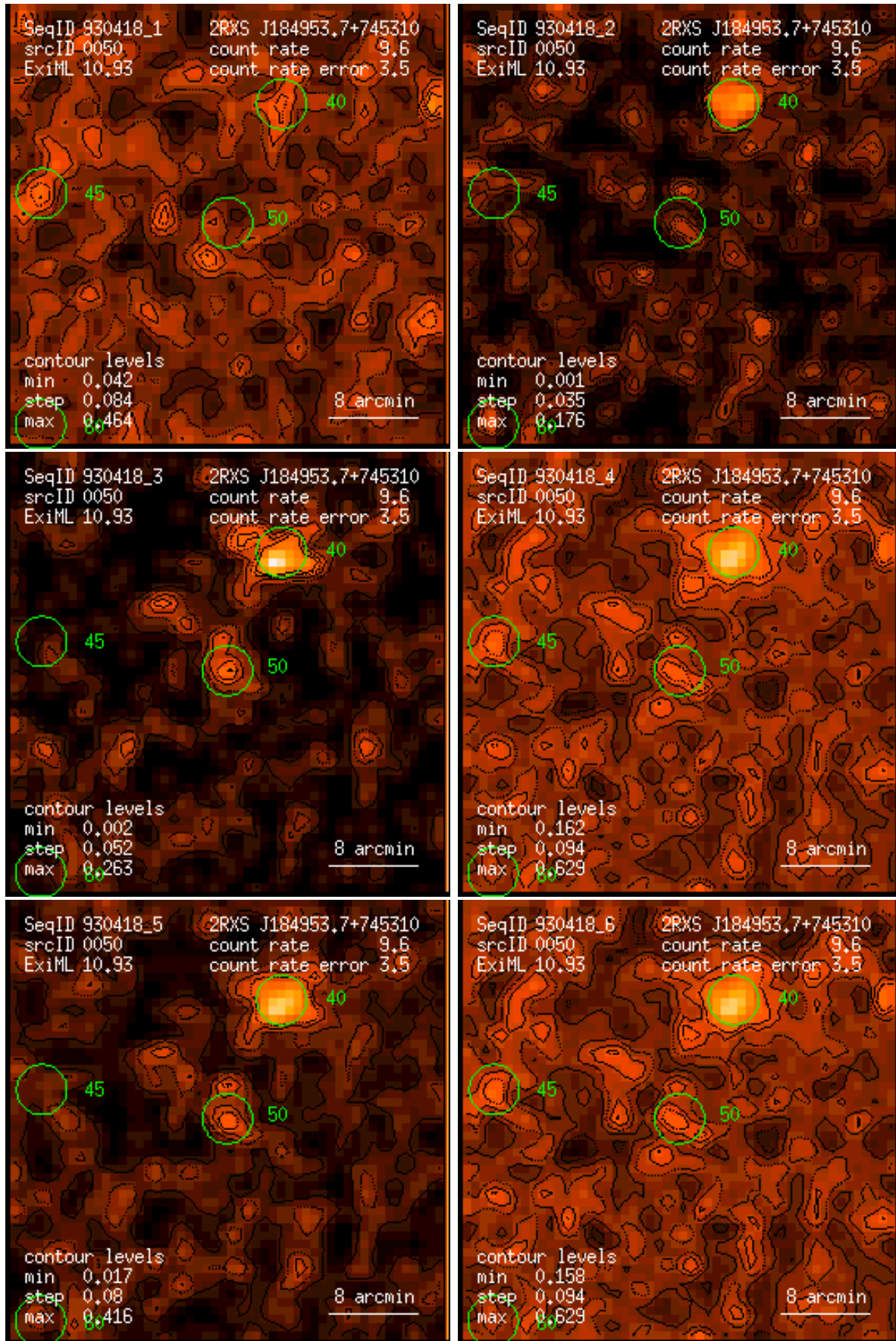
Figure 50: RASS 930418: detection 0050: band rate images, Gaussian filter: (1) PSPC channels 11 – 41, (2) 52 – 90, (3) 91 – 201, (4) 11 – 235, (5) 52 – 201, (6) 11 – 201. Broad band rates in counts/ks. Band rate contour levels in counts/ks/arcmin 2 .
