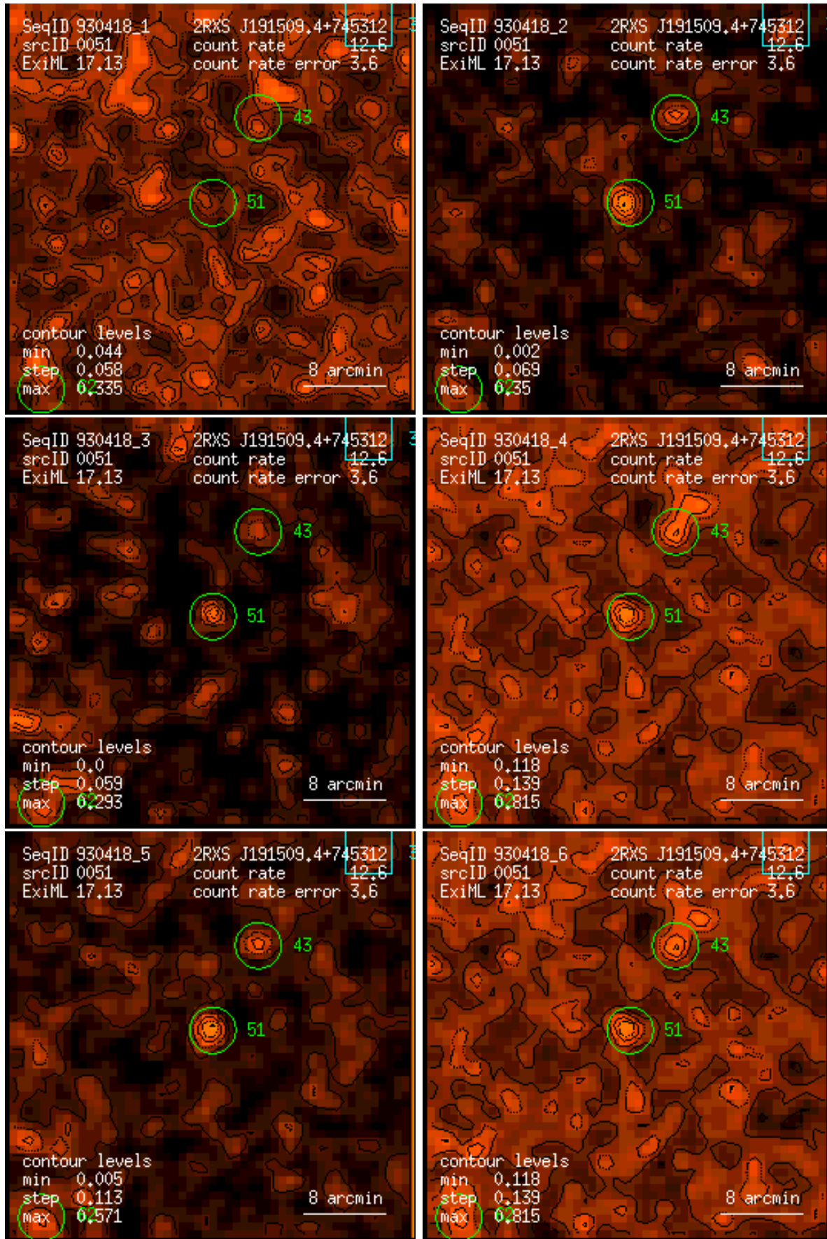
Figure 51: RASS 930418: detection 0051: band rate images, Gaussian filter: (1) PSPC channels 11 – 41, (2) 52 – 90, (3) 91 – 201, (4) 11 – 235, (5) 52 – 201, (6) 11 – 201. Broad band rates in counts/ks. Band rate contour levels in counts/ks/arcmin 2 .
