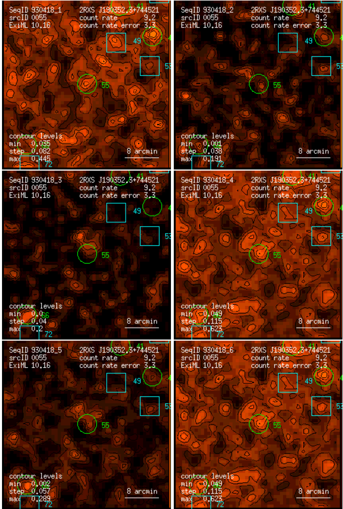
Figure 55: RASS 930418: detection 0055: band rate images, Gaussian filter: (1) PSPC channels 11 – 41, (2) 52 – 90, (3) 91 – 201, (4) 11 – 235, (5) 52 – 201, (6) 11 – 201. Broad band rates in counts/ks. Band rate contour levels in counts/ks/arcmin 2 .
