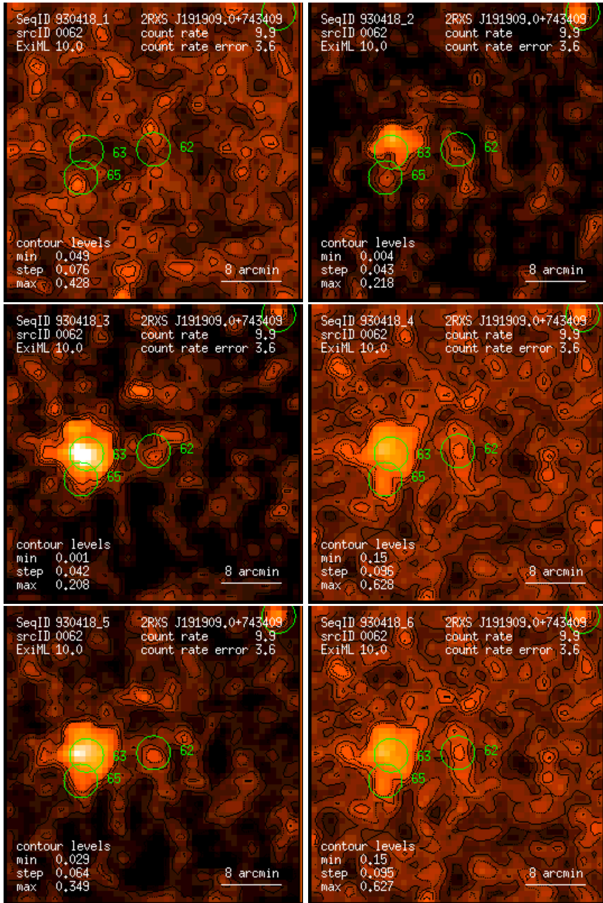
Figure 62: RASS 930418: detection 0062: band rate images, Gaussian filter: (1) PSPC channels 11 – 41, (2) 52 – 90, (3) 91 – 201, (4) 11 – 235, (5) 52 – 201, (6) 11 – 201. Broad band rates in counts/ks. Band rate contour levels in counts/ks/arcmin 2 .
