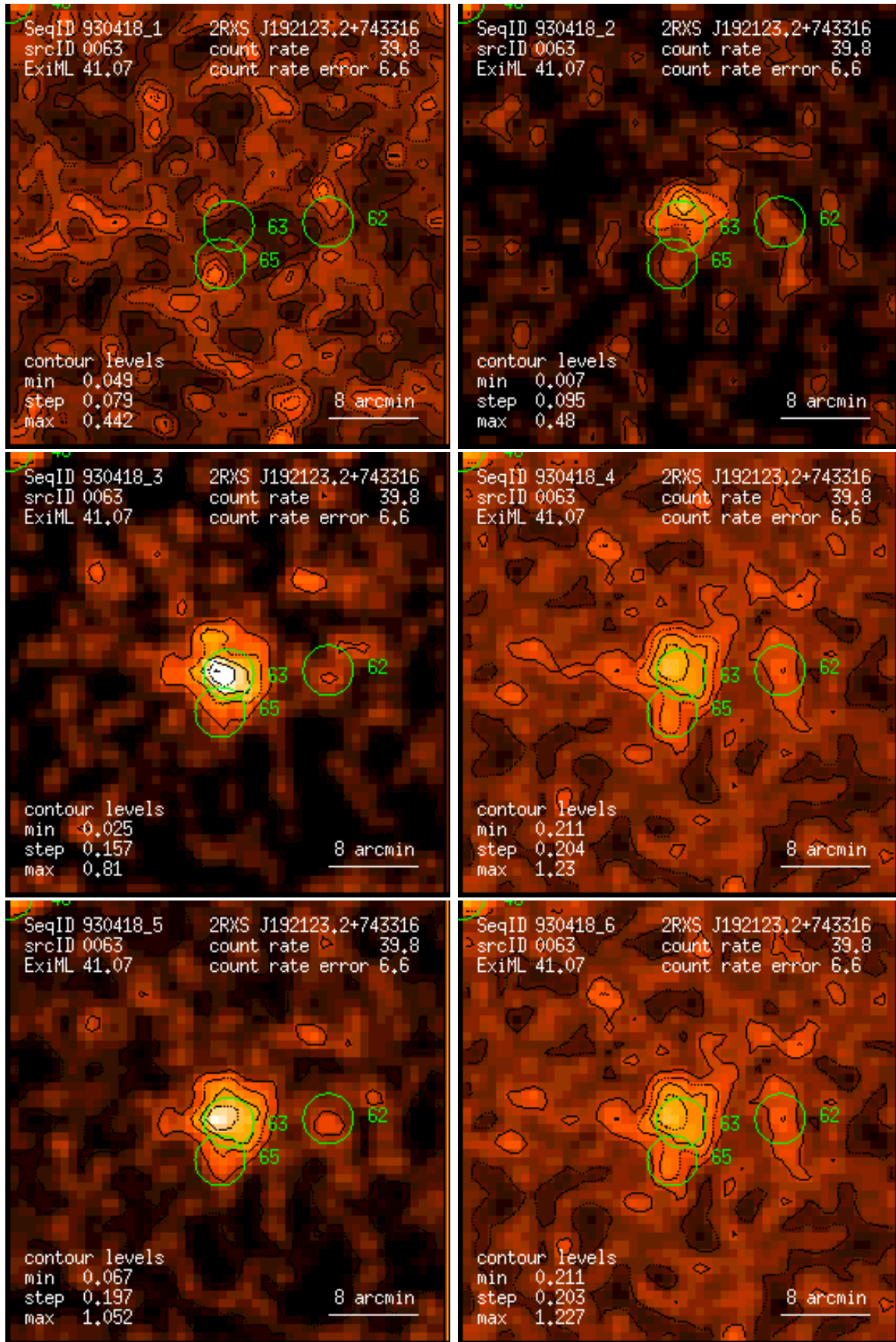
Figure 63: RASS 930418: detection 0063: band rate images, Gaussian filter: (1) PSPC channels 11 – 41, (2) 52 – 90, (3) 91 – 201, (4) 11 – 235, (5) 52 – 201, (6) 11 – 201. Broad band rates in counts/ks. Band rate contour levels in counts/ks/arcmin 2 .
