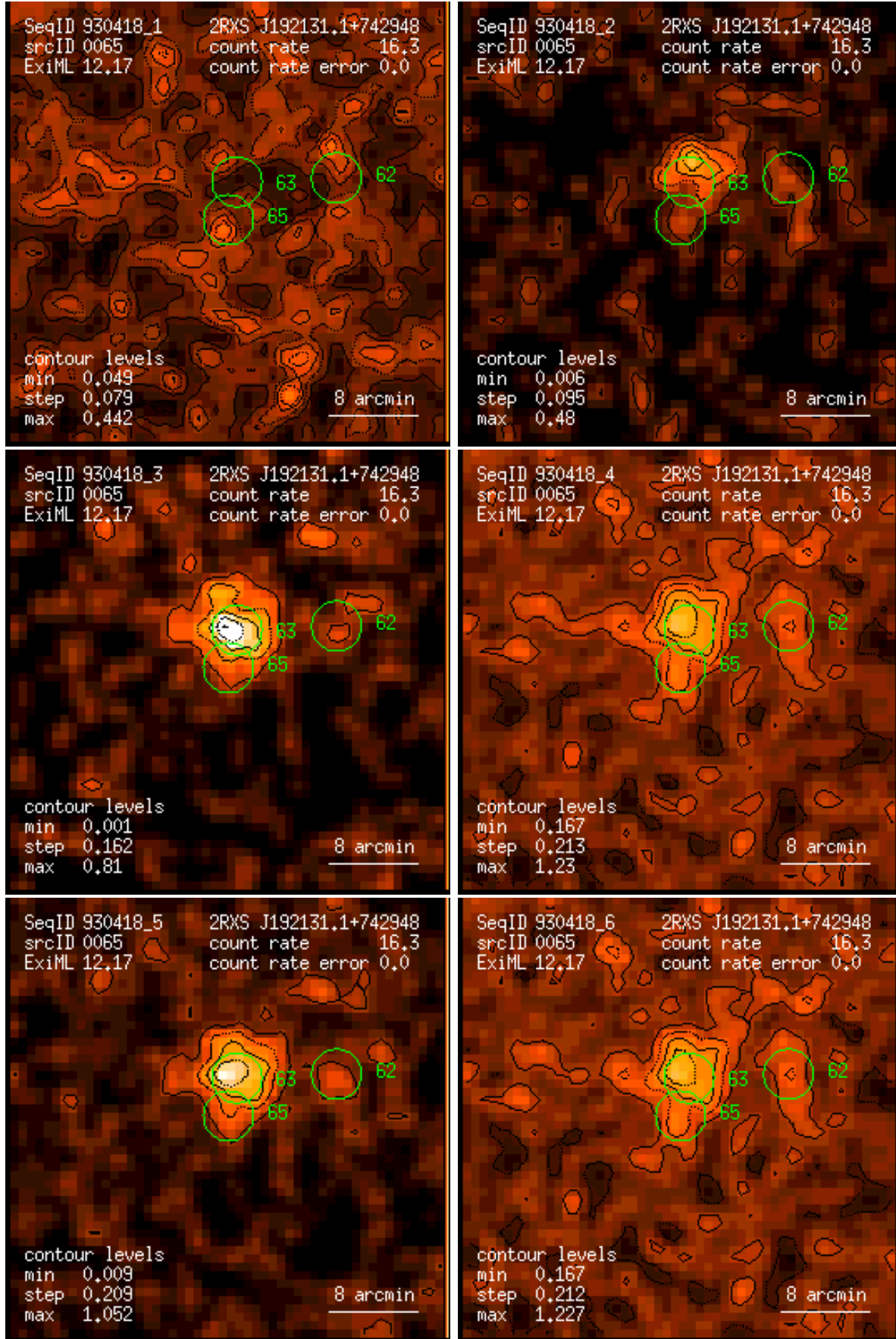
Figure 65: RASS 930418: detection 0065: band rate images, Gaussian filter: (1) PSPC channels 11 – 41, (2) 52 – 90, (3) 91 – 201, (4) 11 – 235, (5) 52 – 201, (6) 11 – 201. Broad band rates in counts/ks. Band rate contour levels in counts/ks/arcmin 2 .
