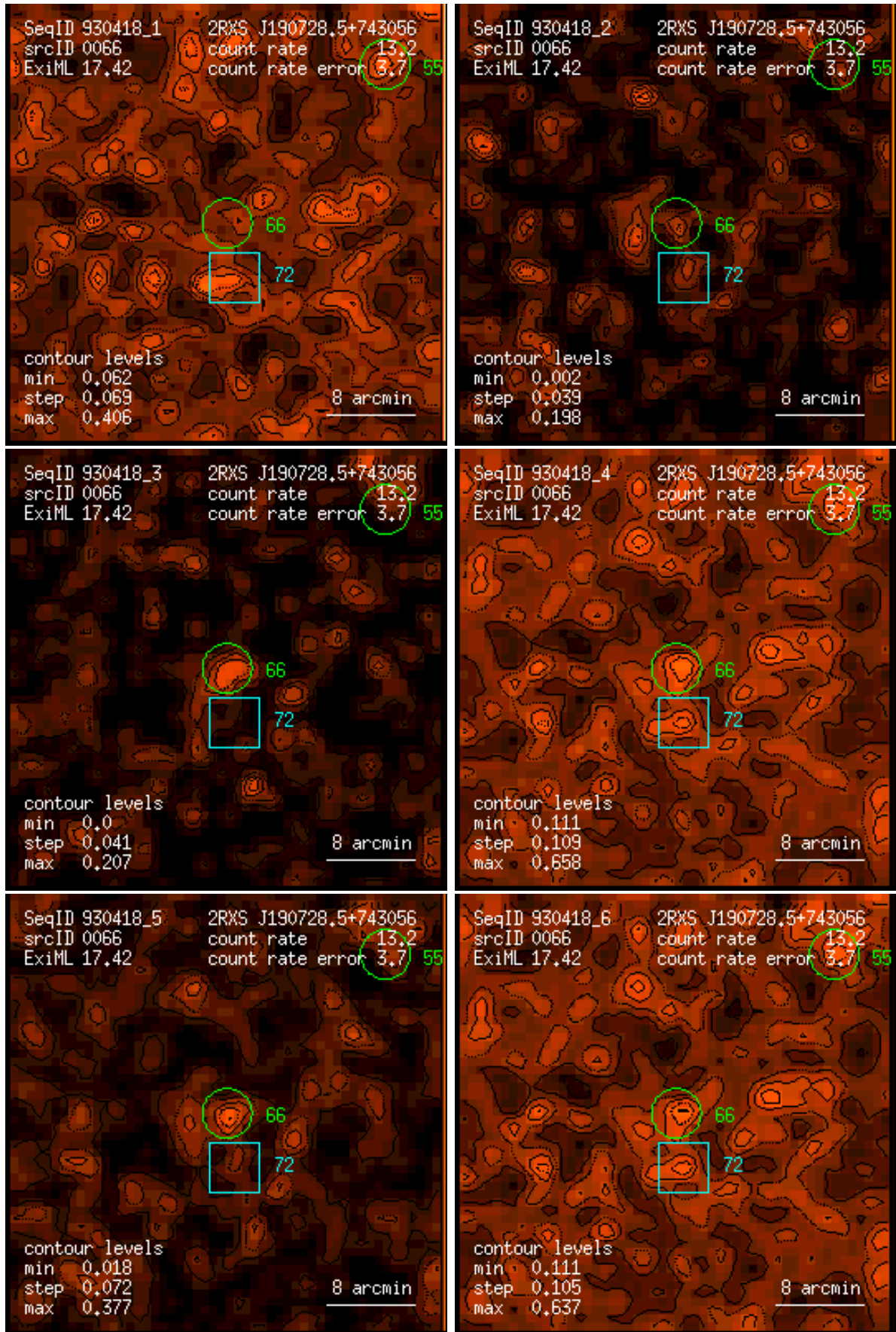
Figure 66: RASS 930418: detection 0066: band rate images, Gaussian filter: (1) PSPC channels 11 – 41, (2) 52 – 90, (3) 91 – 201, (4) 11 – 235, (5) 52 – 201, (6) 11 – 201. Broad band rates in counts/ks. Band rate contour levels in counts/ks/arcmin 2 .
