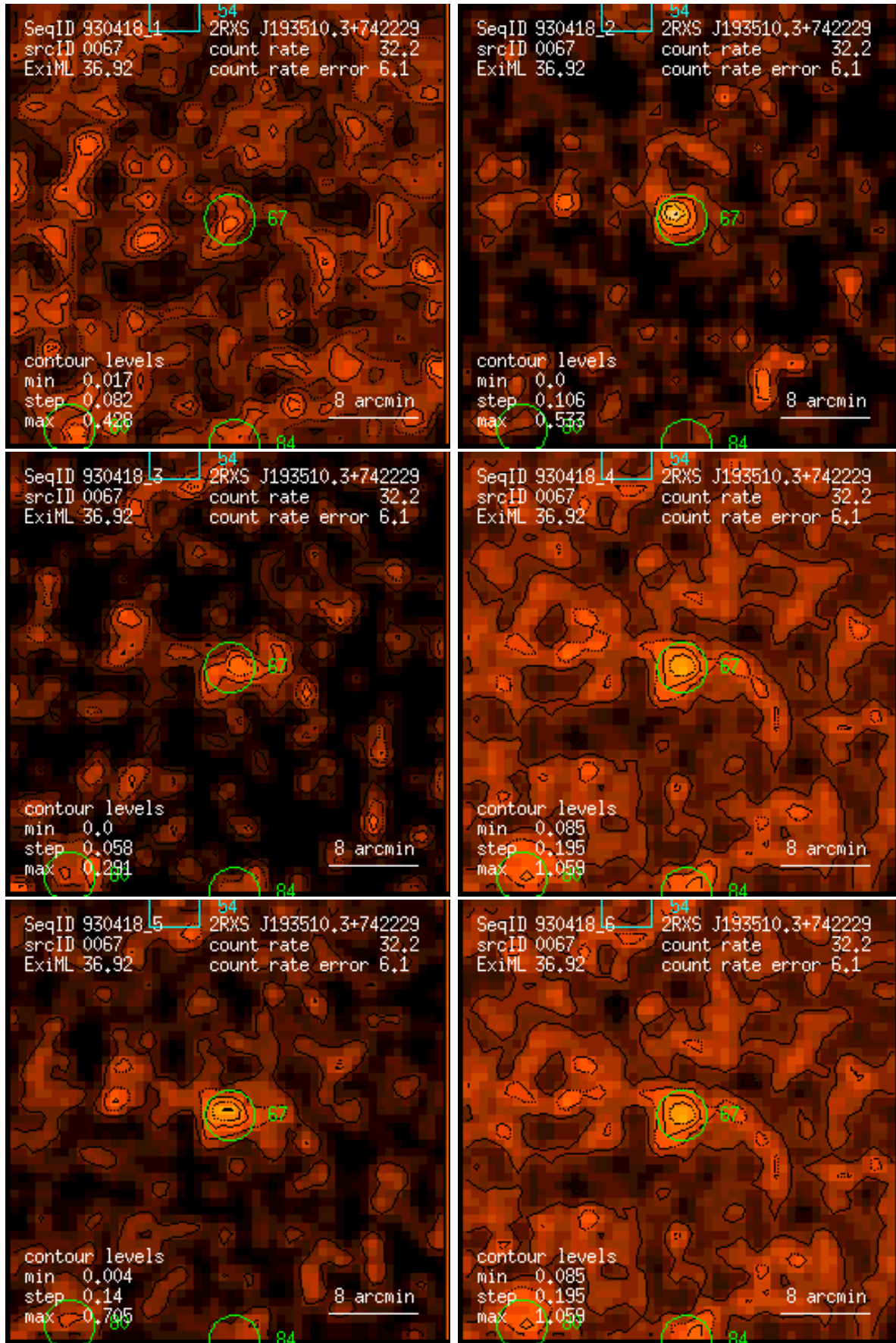
Figure 67: RASS 930418: detection 0067: band rate images, Gaussian filter: (1) PSPC channels 11 – 41, (2) 52 – 90, (3) 91 – 201, (4) 11 – 235, (5) 52 – 201, (6) 11 – 201. Broad band rates in counts/ks. Band rate contour levels in counts/ks/arcmin 2 .
