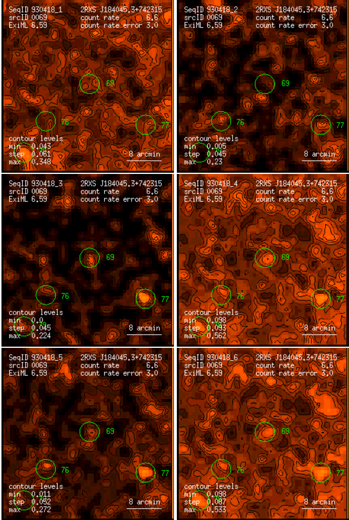
Figure 69: RASS 930418: detection 0069: band rate images, Gaussian filter: (1) PSPC channels 11 – 41, (2) 52 – 90, (3) 91 – 201, (4) 11 – 235, (5) 52 – 201, (6) 11 – 201. Broad band rates in counts/ks. Band rate contour levels in counts/ks/arcmin 2 .
